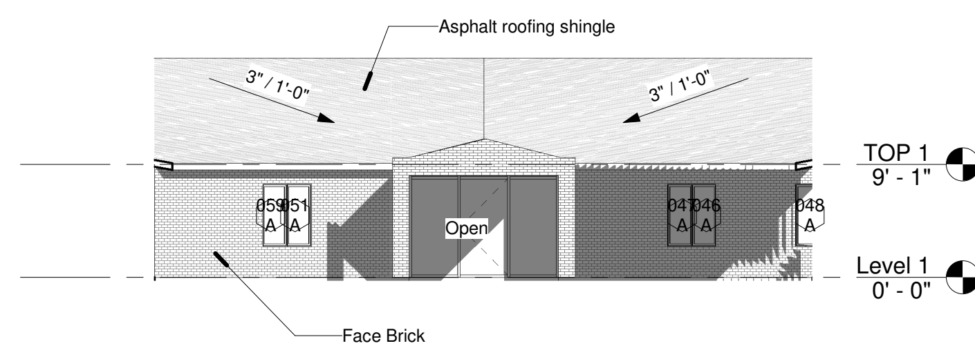
⑤ Main Entry 3/32" = 1'-0"
