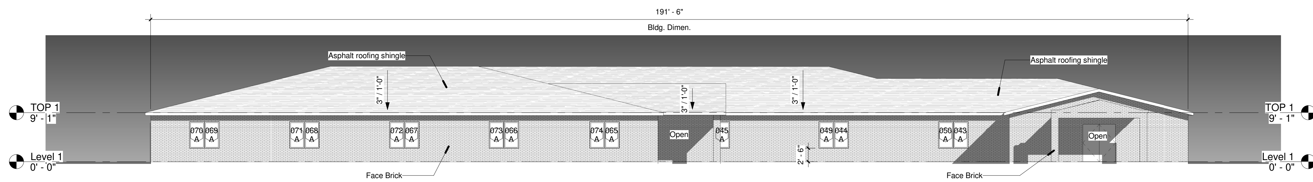
④ West Elevation 3/32" = 1'-0"
