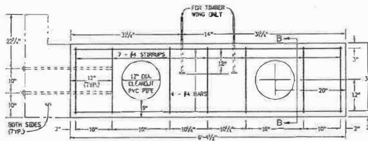
ELEVATION OF LATERAL SUPPORT
