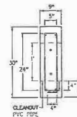
LATERAL SUPPORT SECTION B-B
