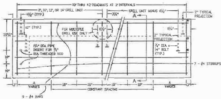
CAST-IN-PLACE FOUNDATION
