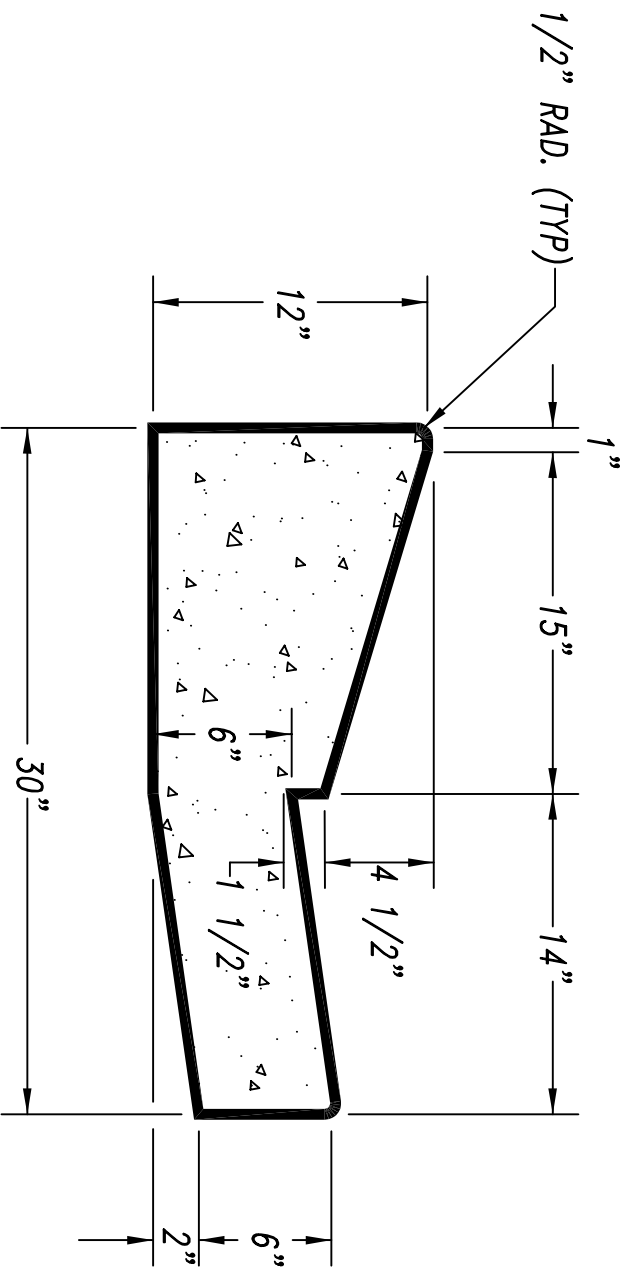
TYPICAL X-SECTION NOT TO SCALE
