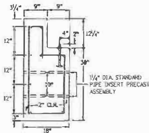
END SECTION OF FOUNDATION SECTION A-A
