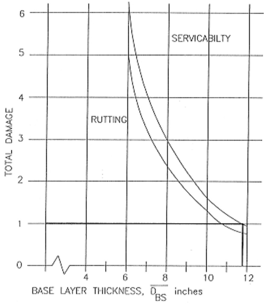
TOTAL DAMAGE VS LAYER THICKNESS GRAPH
