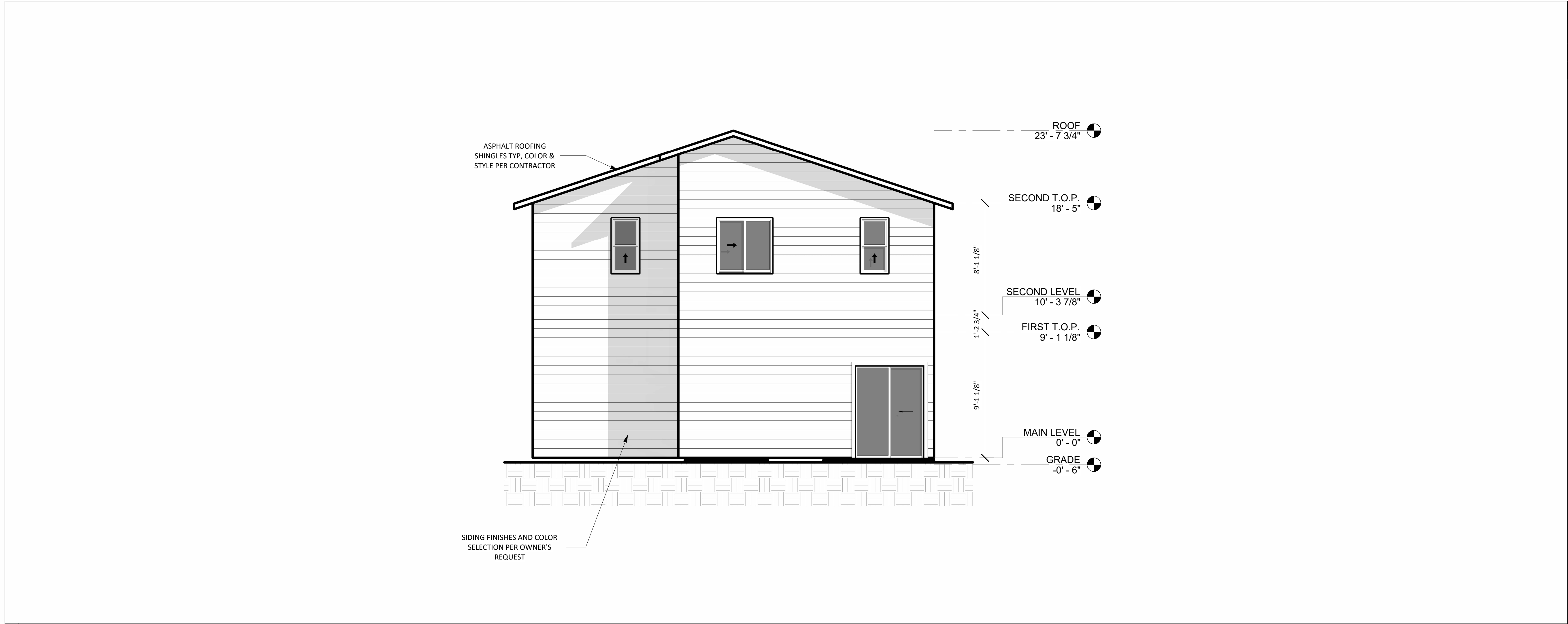
1 REAR ELEVATION 1/4" = 1'-0"
