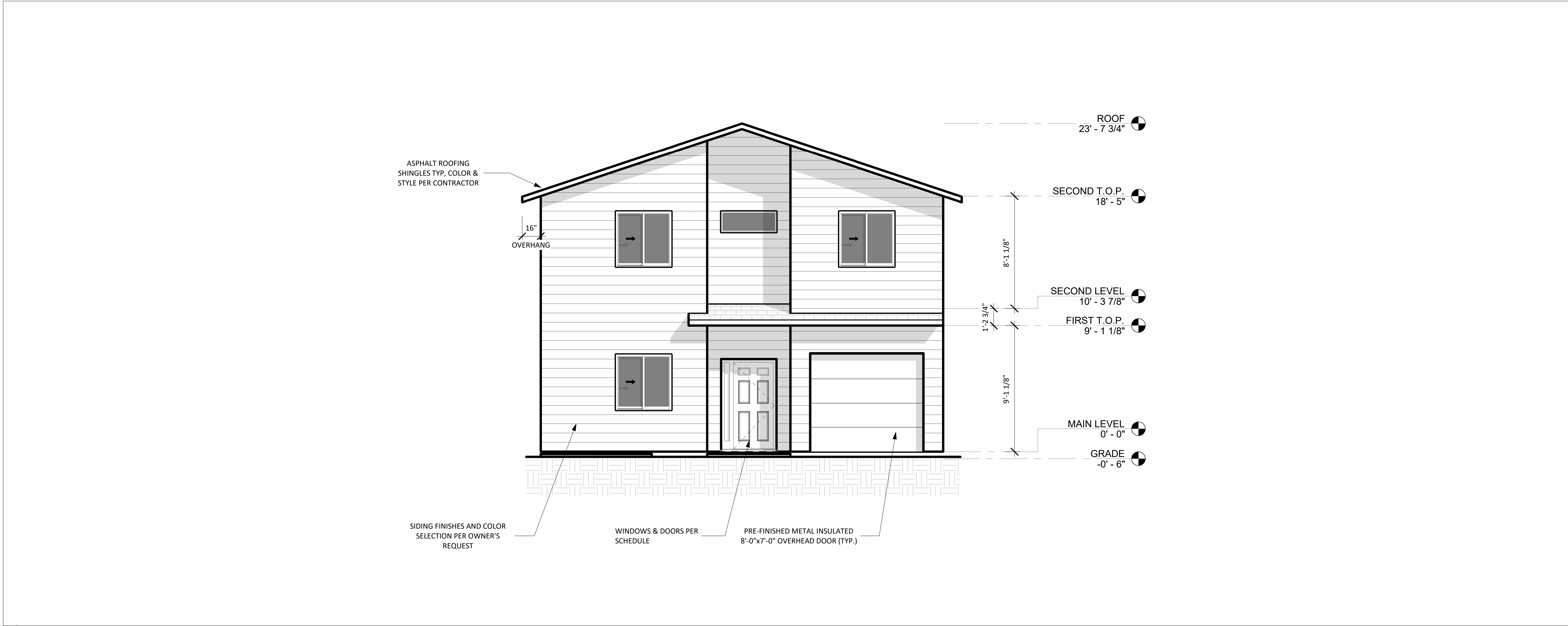
1 FRONT ELEVATION 1/4" = 1'-0"
