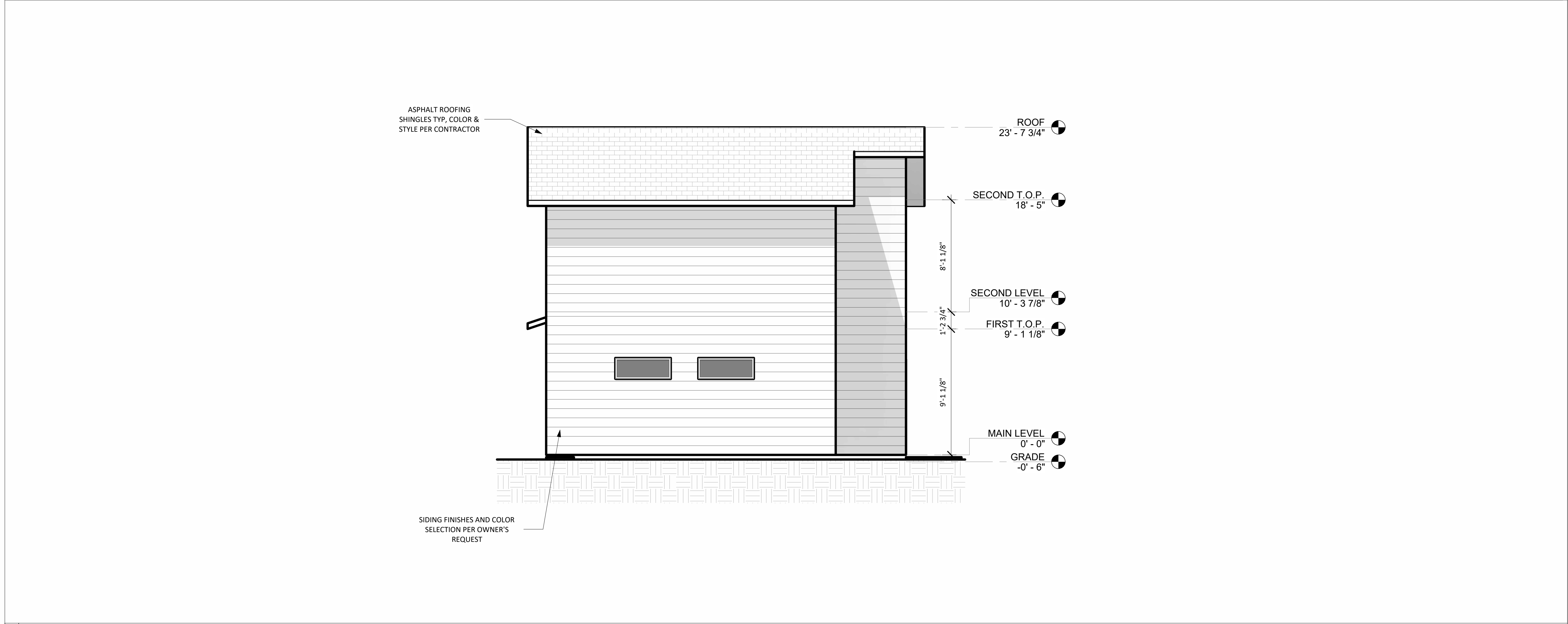
2 LEFT ELEVATION 1/4" = 1'-0"
