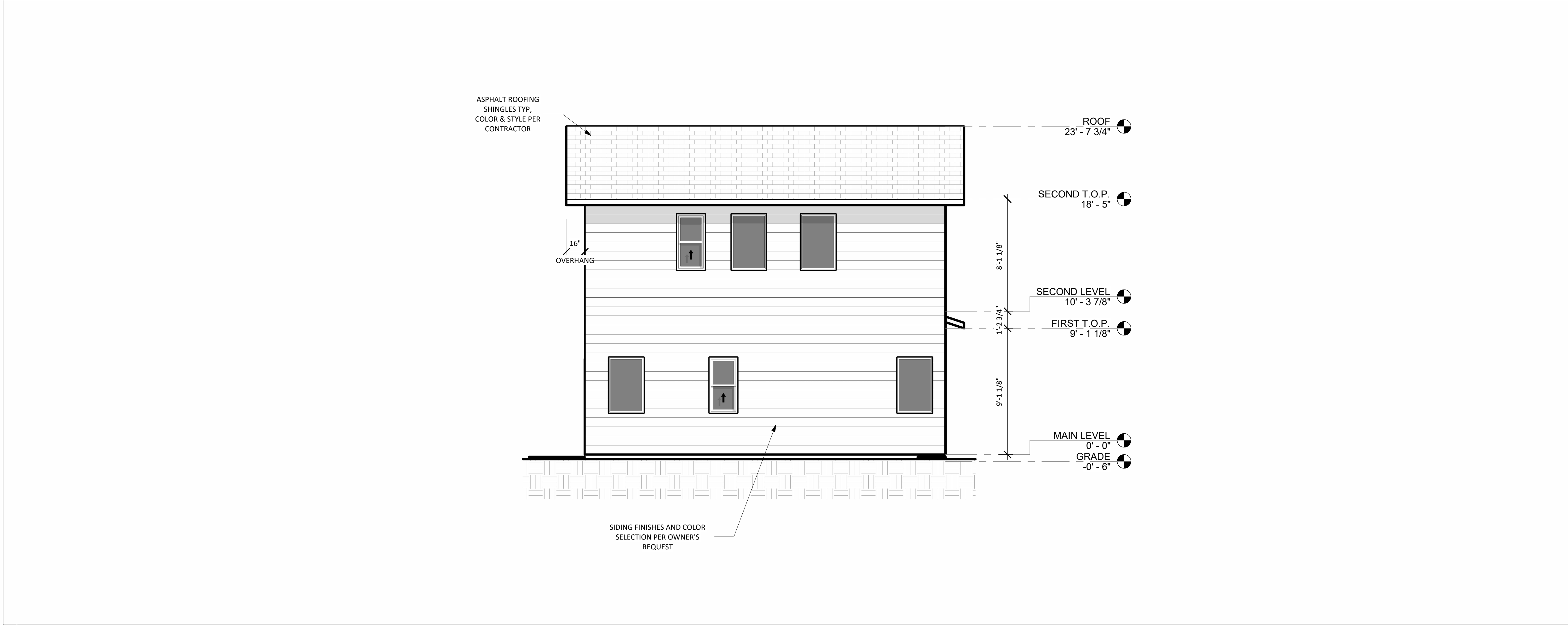
2 RIGHT ELEVATION 1/4" = 1'-0"
