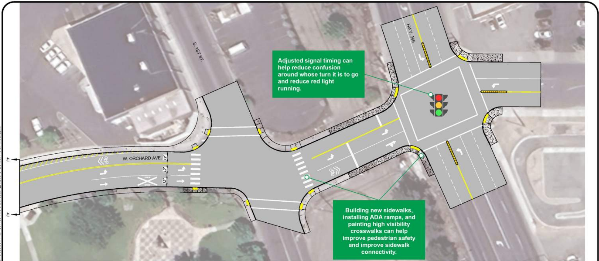
Figure 10. Design concept for Orchard Avenue between OR 207 and US 395 (portion of concept)
