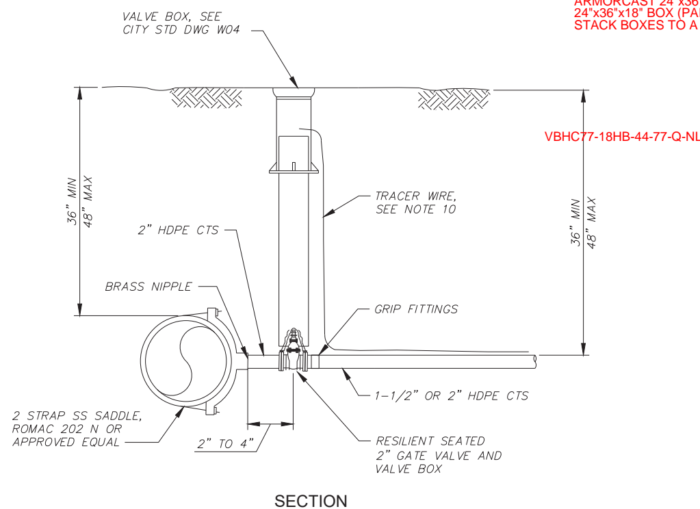
TYPICAL 1-1/2" OR 2" WATER SERVICE LINE
