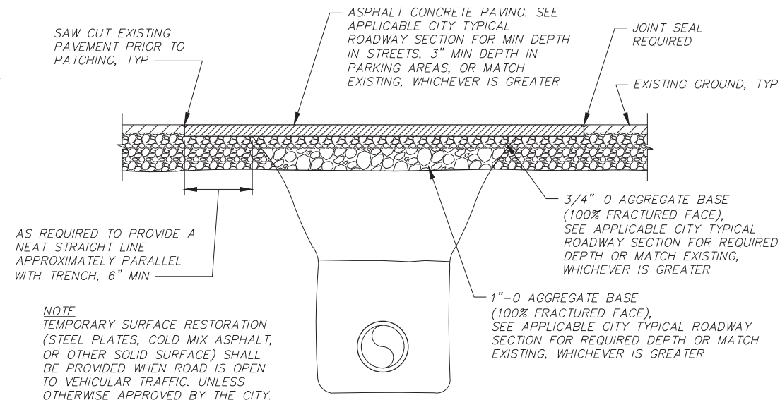
SURFACE RESTORATION PAVED SURFACES
