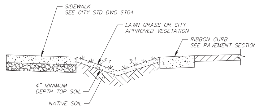
INFILTRATION SWALE OPTION 1
