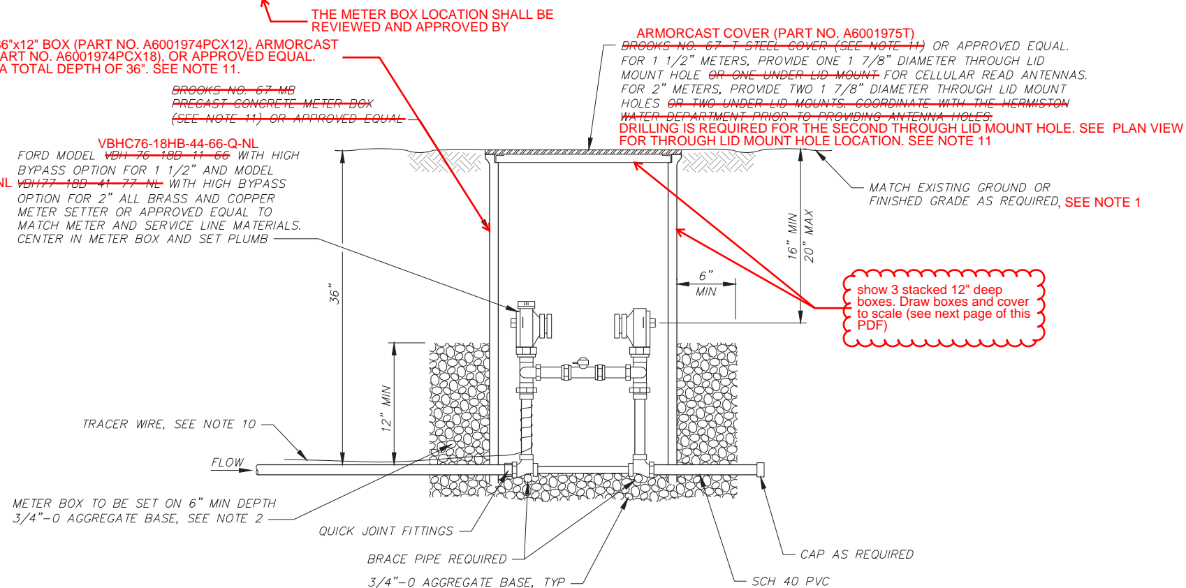
TYPICAL 1-1/2" OR 2" WATER METER INSTALLATION (USING COPPER METERSETTER)
