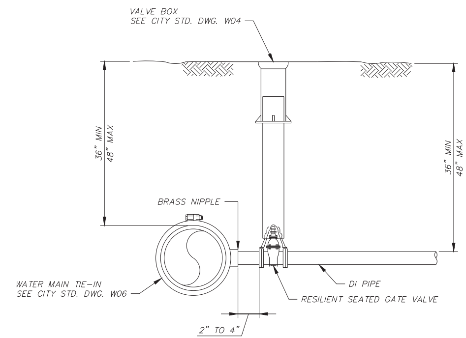
SECTION
