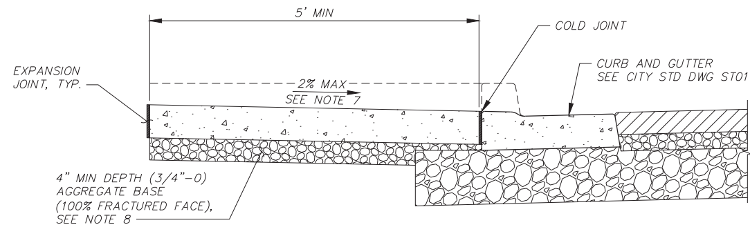
SECTION VIEW
