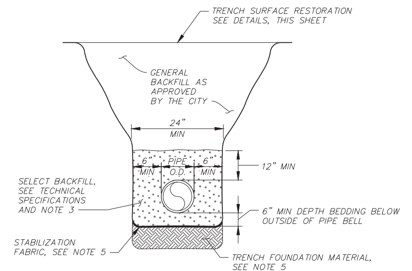
WATER LINE TRENCH BEDDING AND BACKFILL
