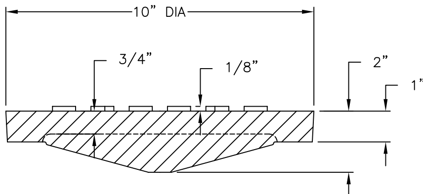
COVER SECTION
