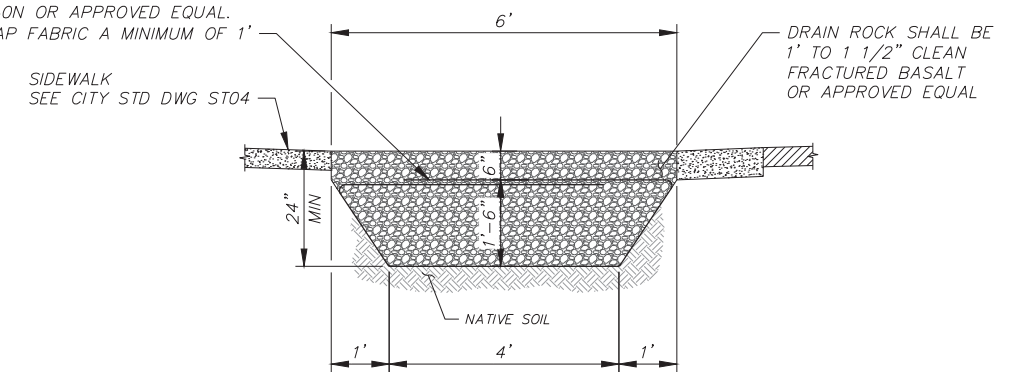
INFILTRATION SWALE OPTION 2
