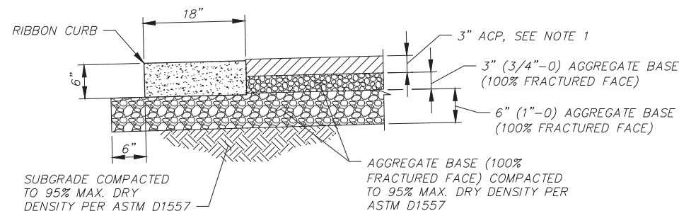
PAVEMENT SECTION
