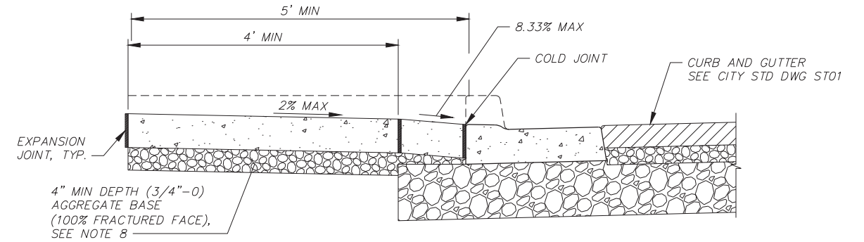
SECTION VIEW
