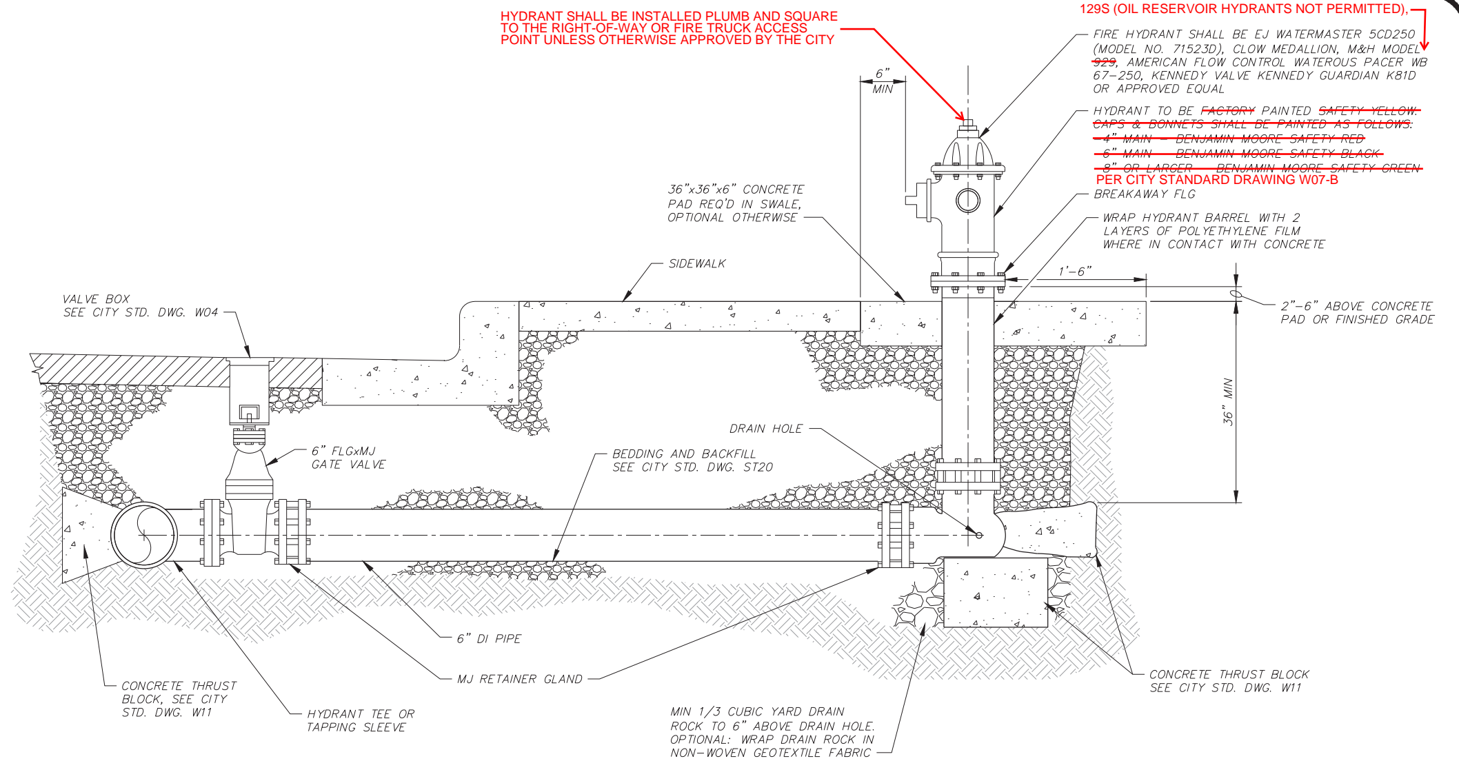
HYDRANT ASSEMBLY
