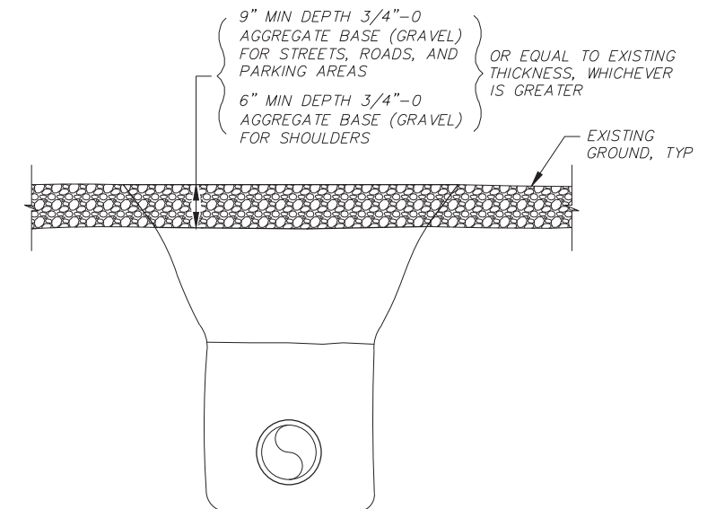
SURFACE RESTORATION GRAVEL SURFACES
