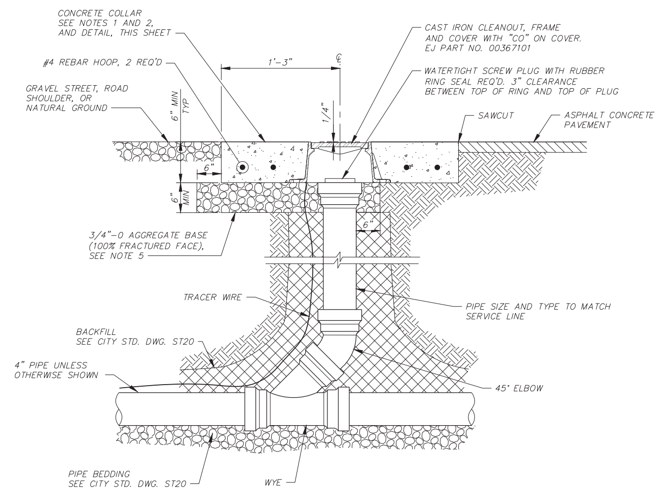
SEWER SERVICE LINE CLEANOUT NTS
