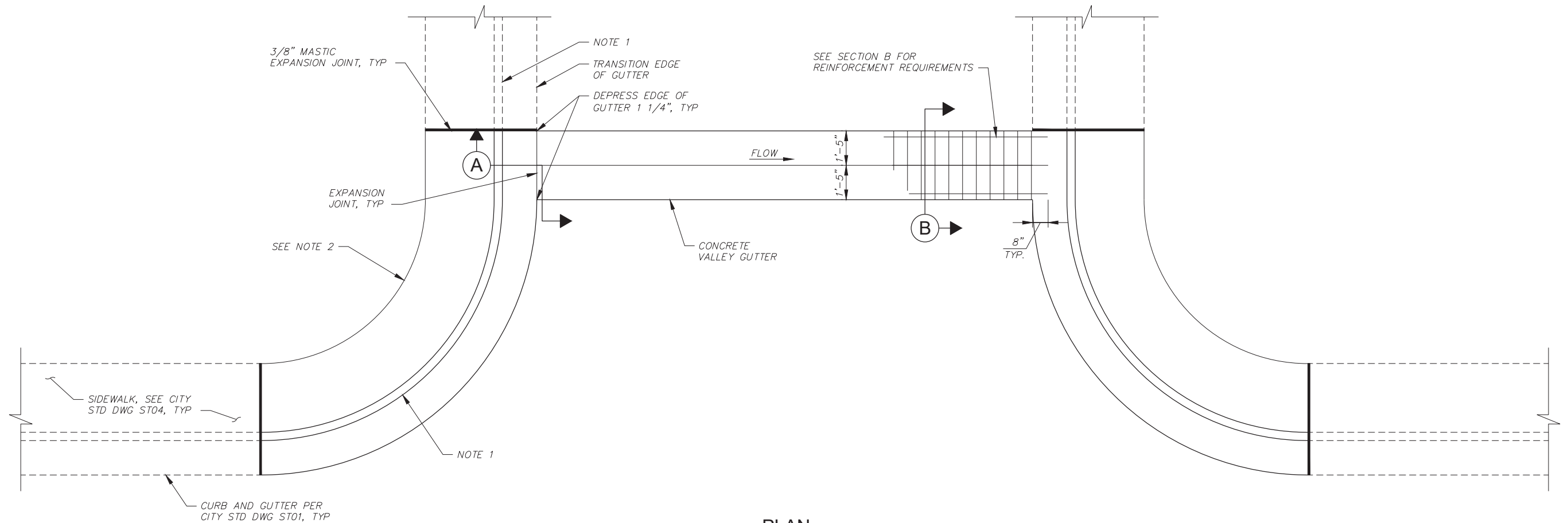
PLAN NTS
