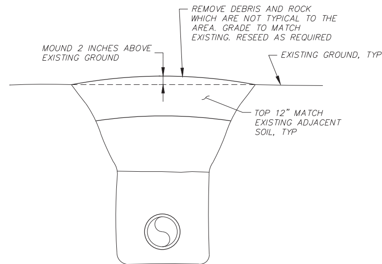
SURFACE RESTORATION NATURAL SURFACES
