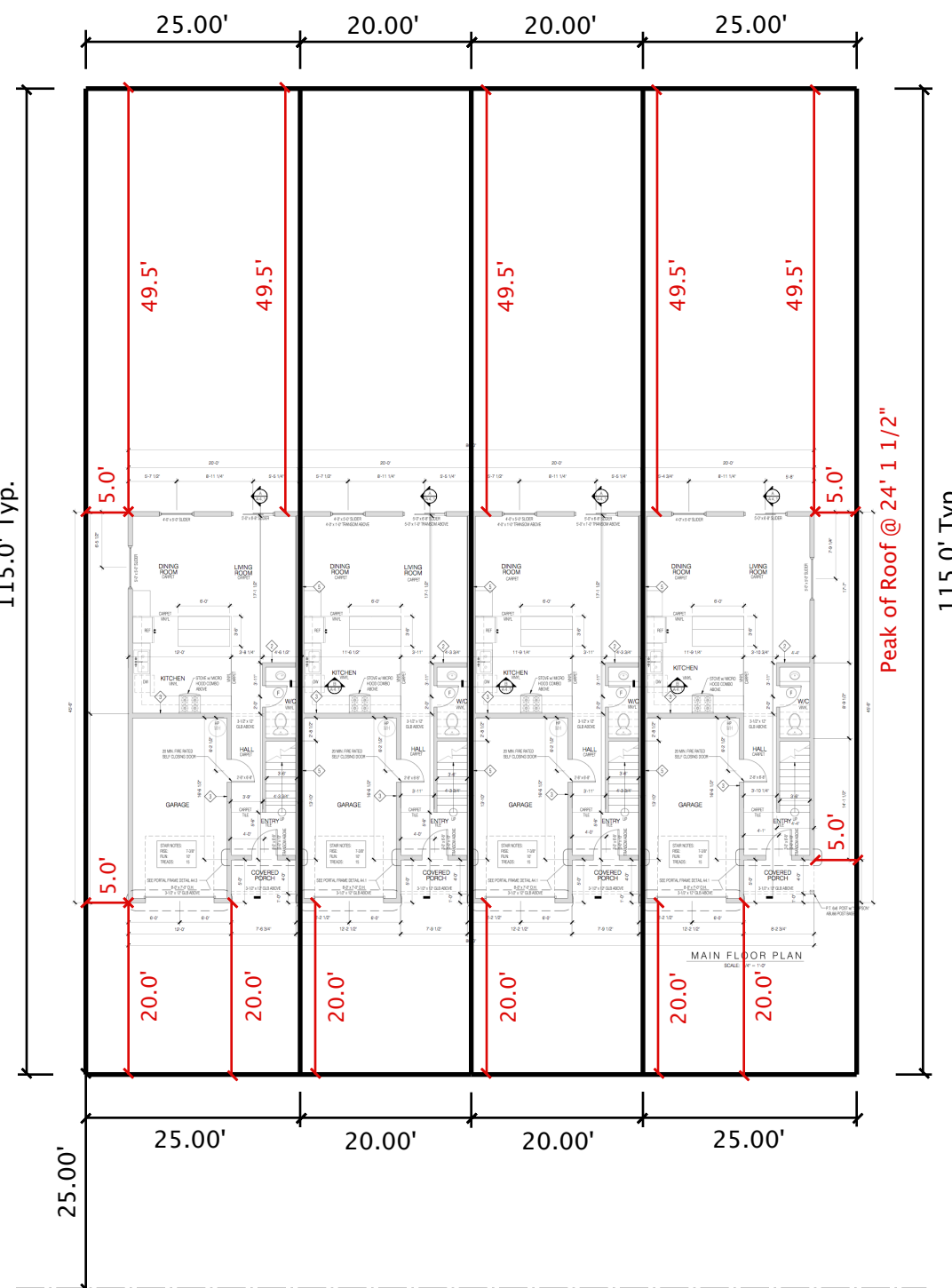
C.L. STREET MESA TYPICAL SCALE 1"=20'
