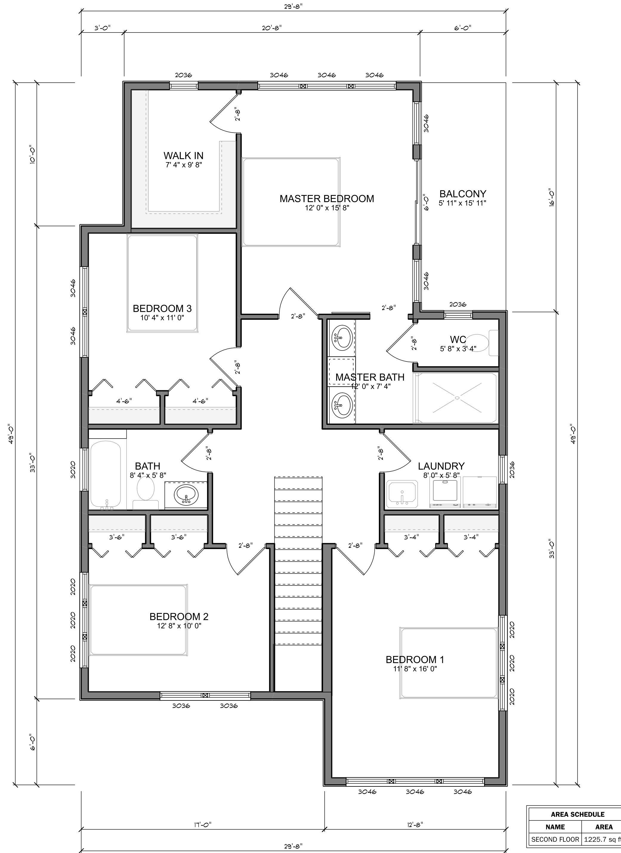
PROPOSED SECOND FLOOR SCALE: 1/4" = 1'-0"
