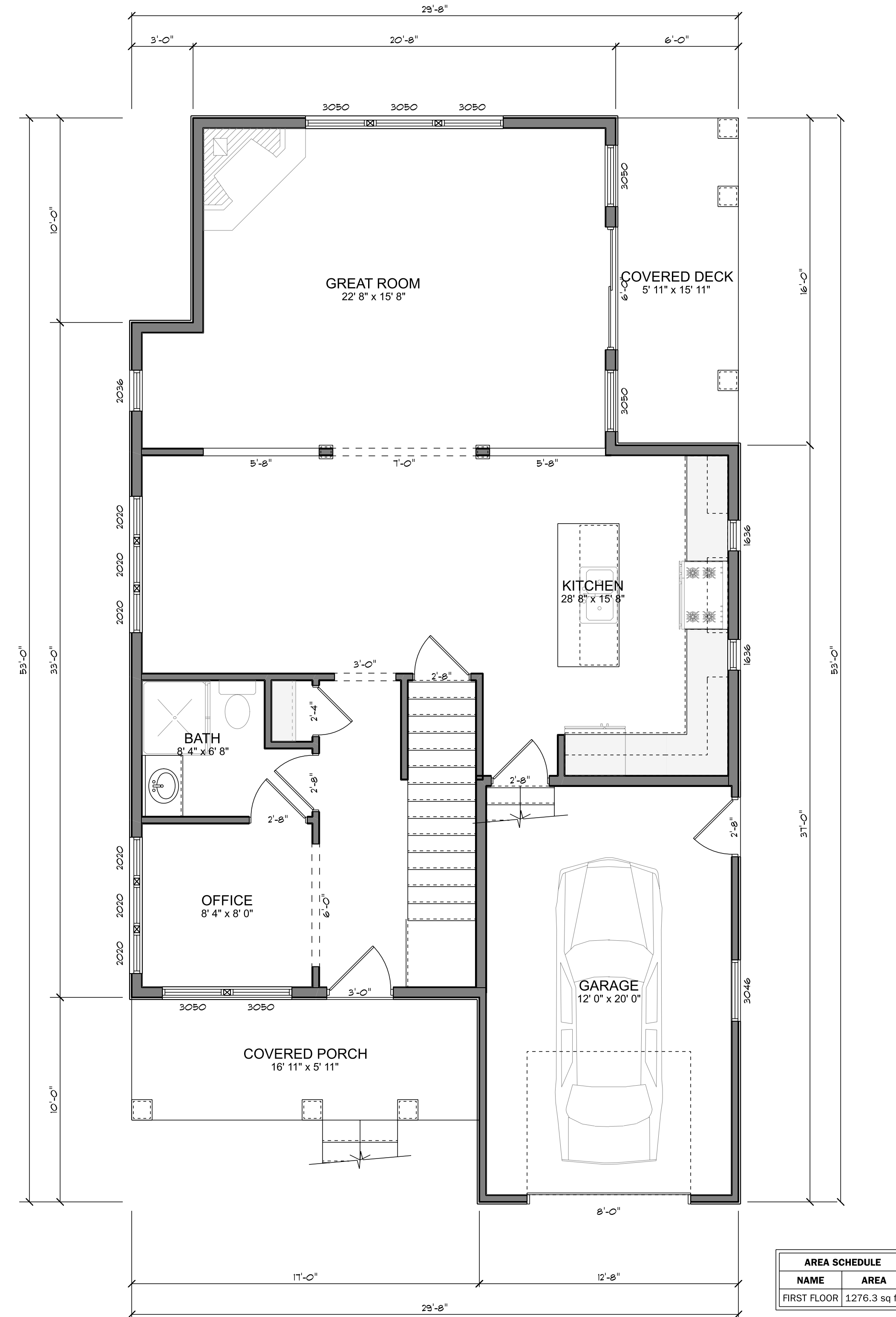
PROPOSED FIRST FLOOR SCALE: 1/4" = 1'-0"
