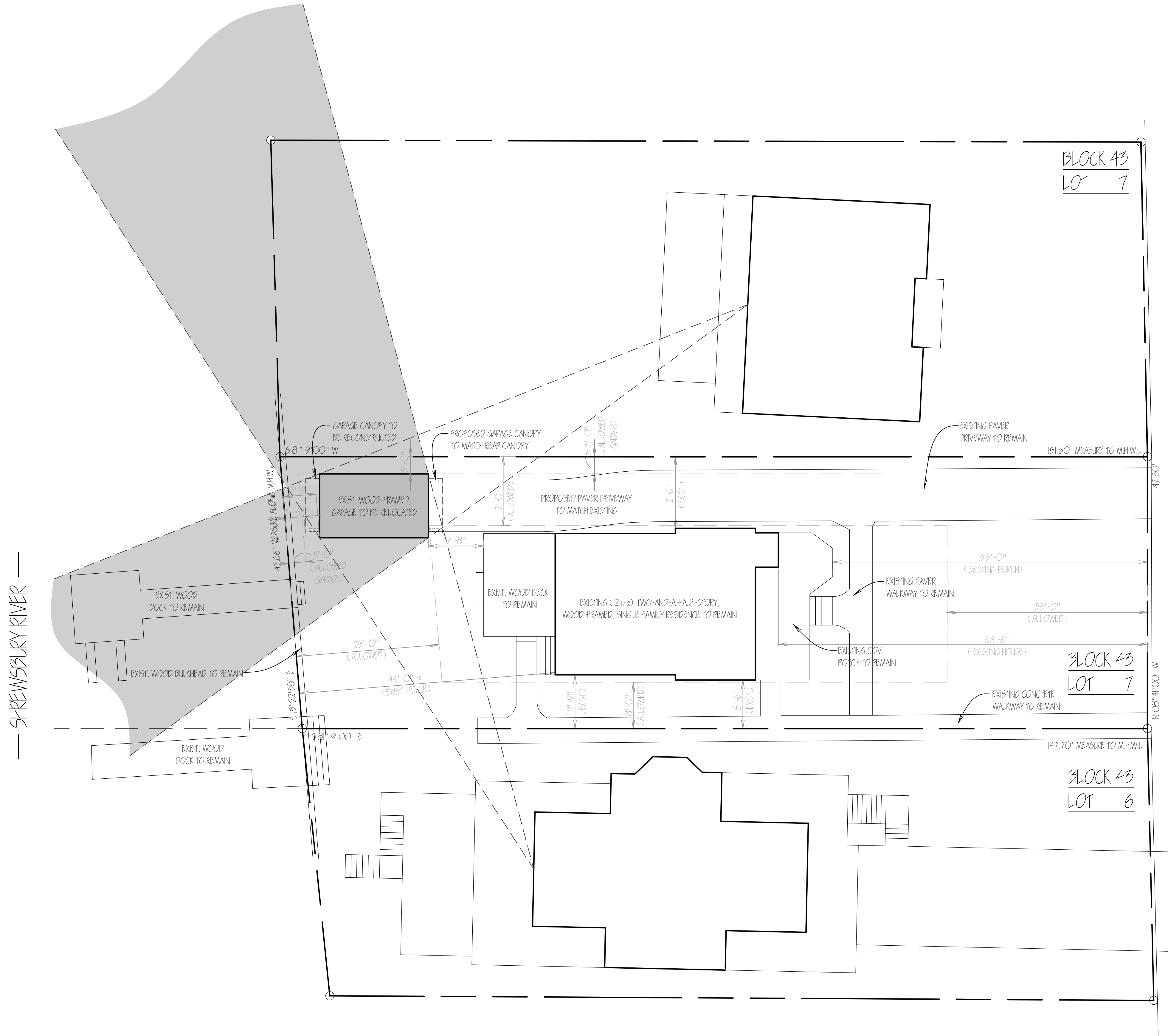
PLOT PLAN ~ VIEW DIAGRAM "A" SCALE: 1" = 10'-0"
