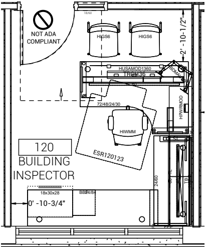
FLOORPLAN
