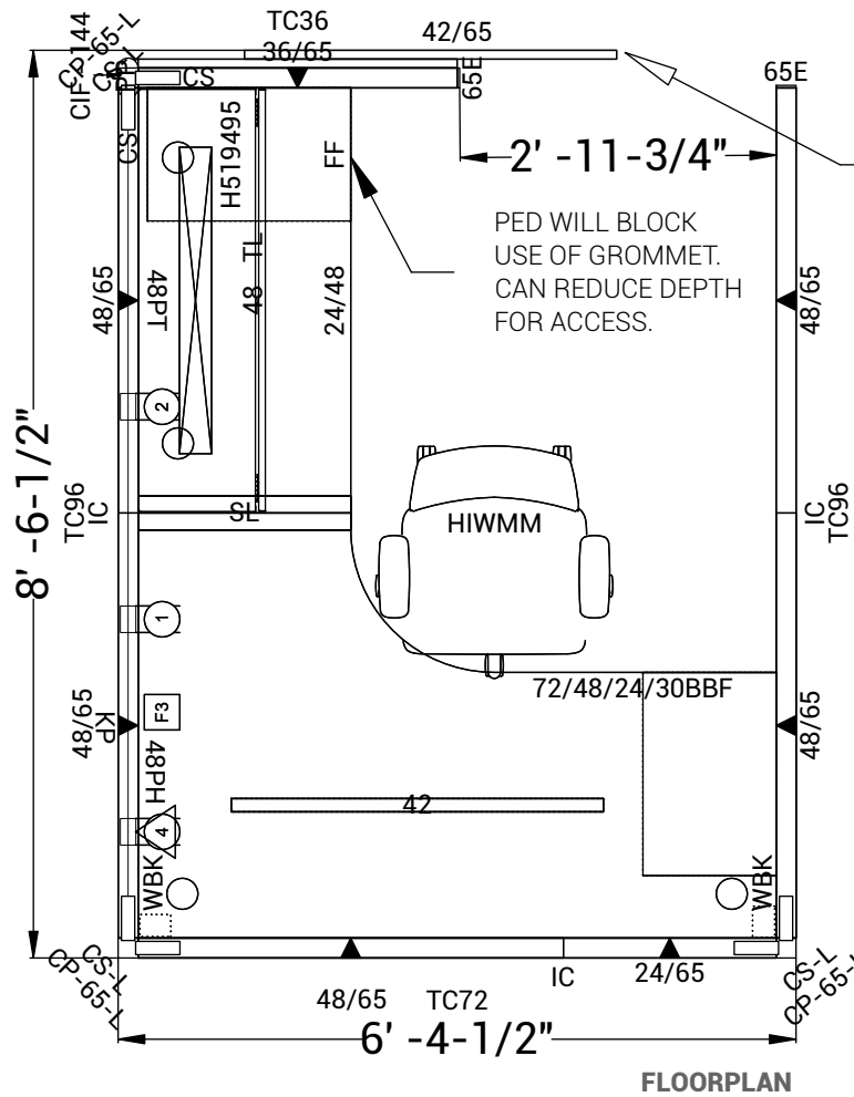
FLOORPLAN
