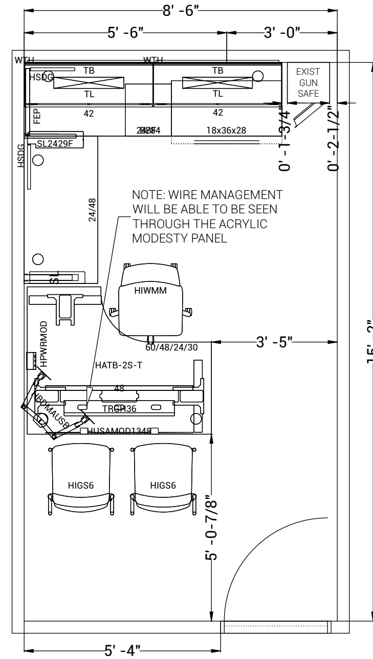
FLOORPLAN
