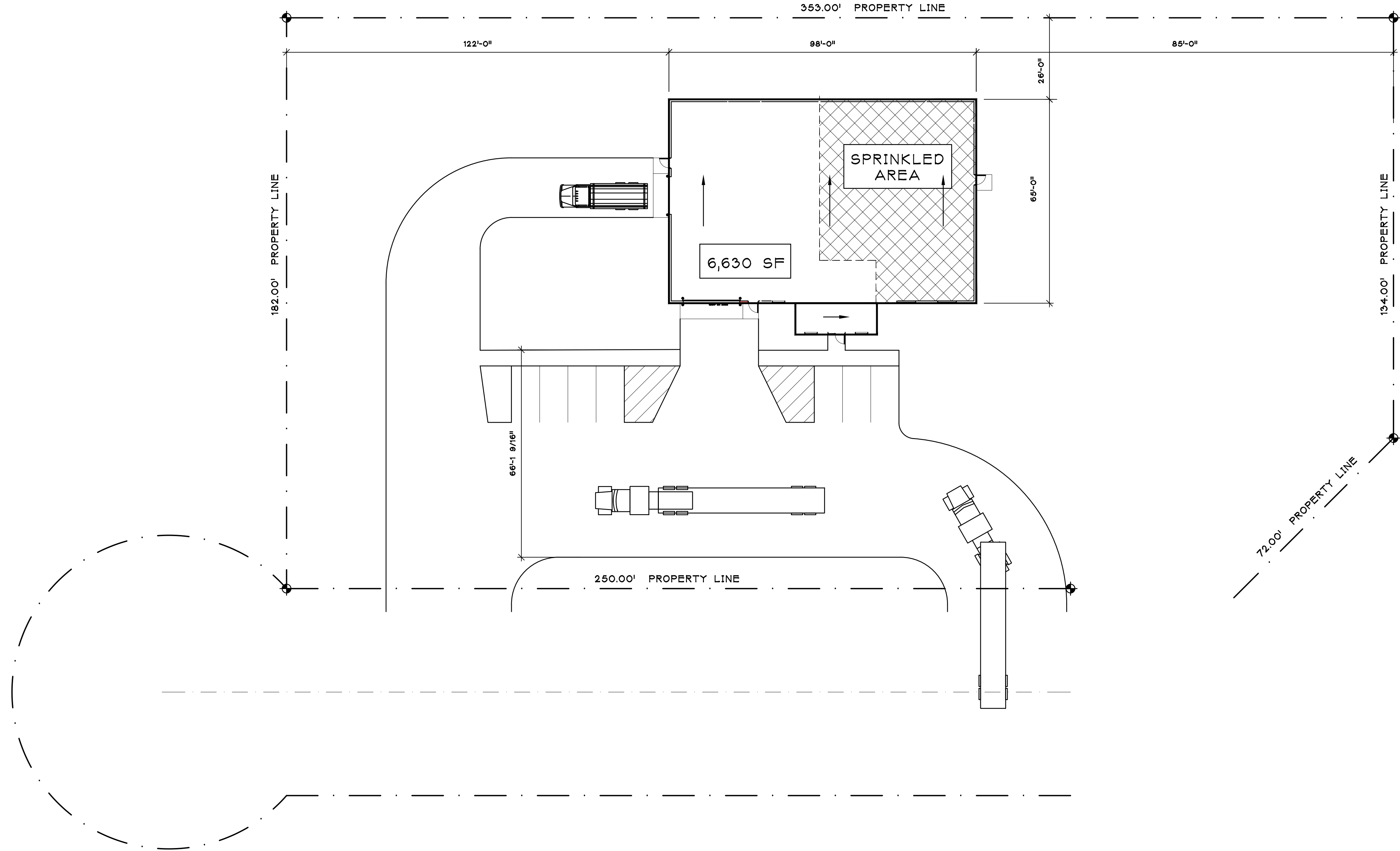
SCHEMATIC SITE PLAN SCALE: 1" = 20'-0"
