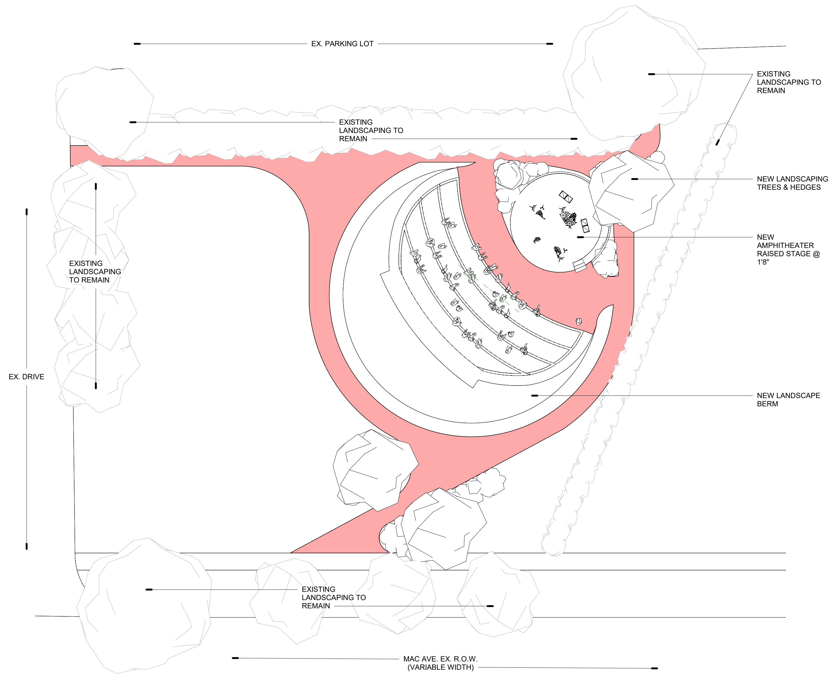
SITE PLAN - NEW AMPHITHEATER
