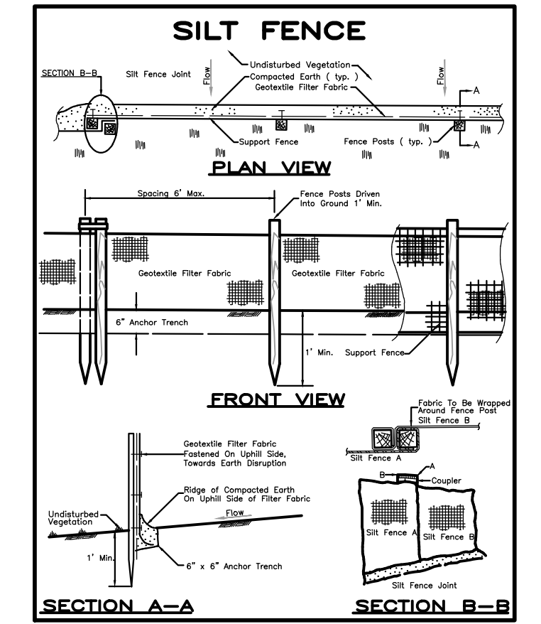
TYPICAL SILT FENCE DETAILS
