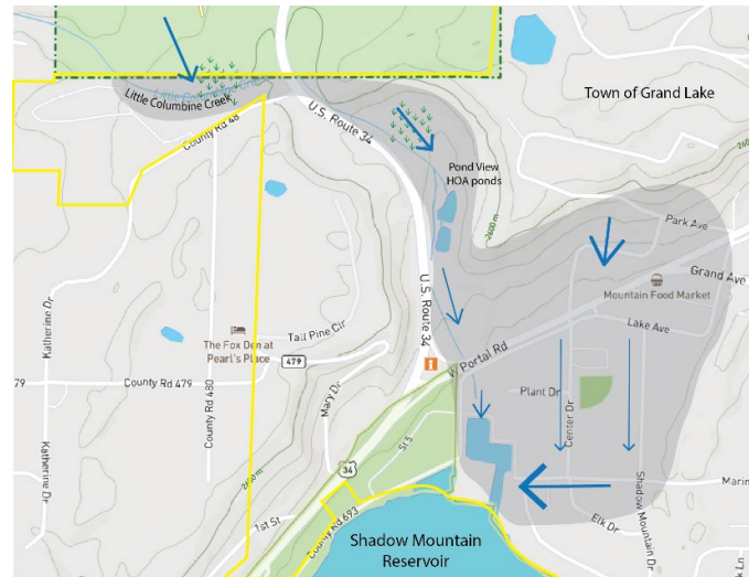
■ Area for potential stormwater management planning → Direction of flow
