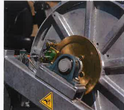
Braking system with electric over hydraulic activation
