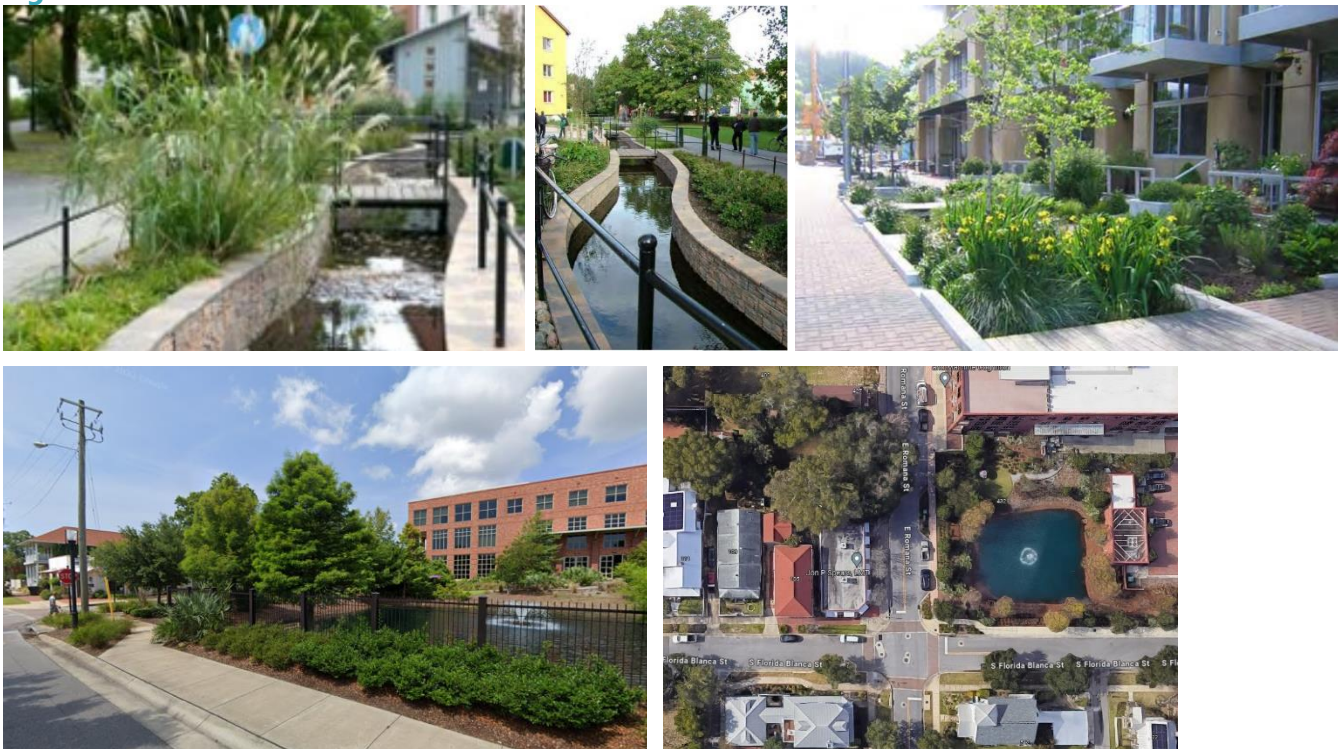
Figure XIV - 59. Alternative Stormwater Detention Facilities
