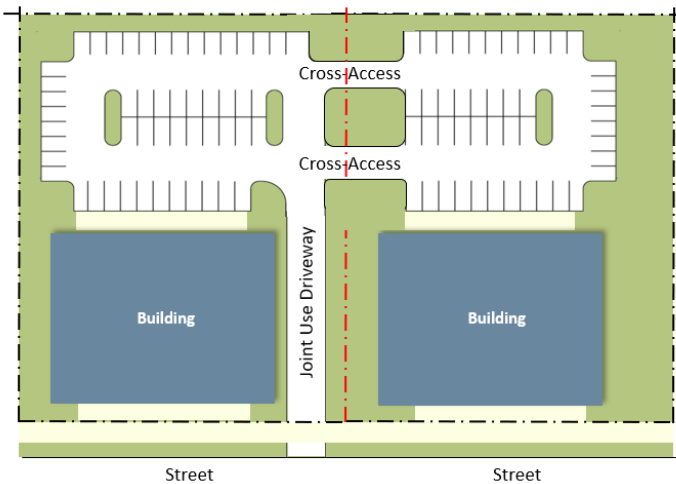
Figure XIV - 51. Joint Use Driveways/Cross-Access.
