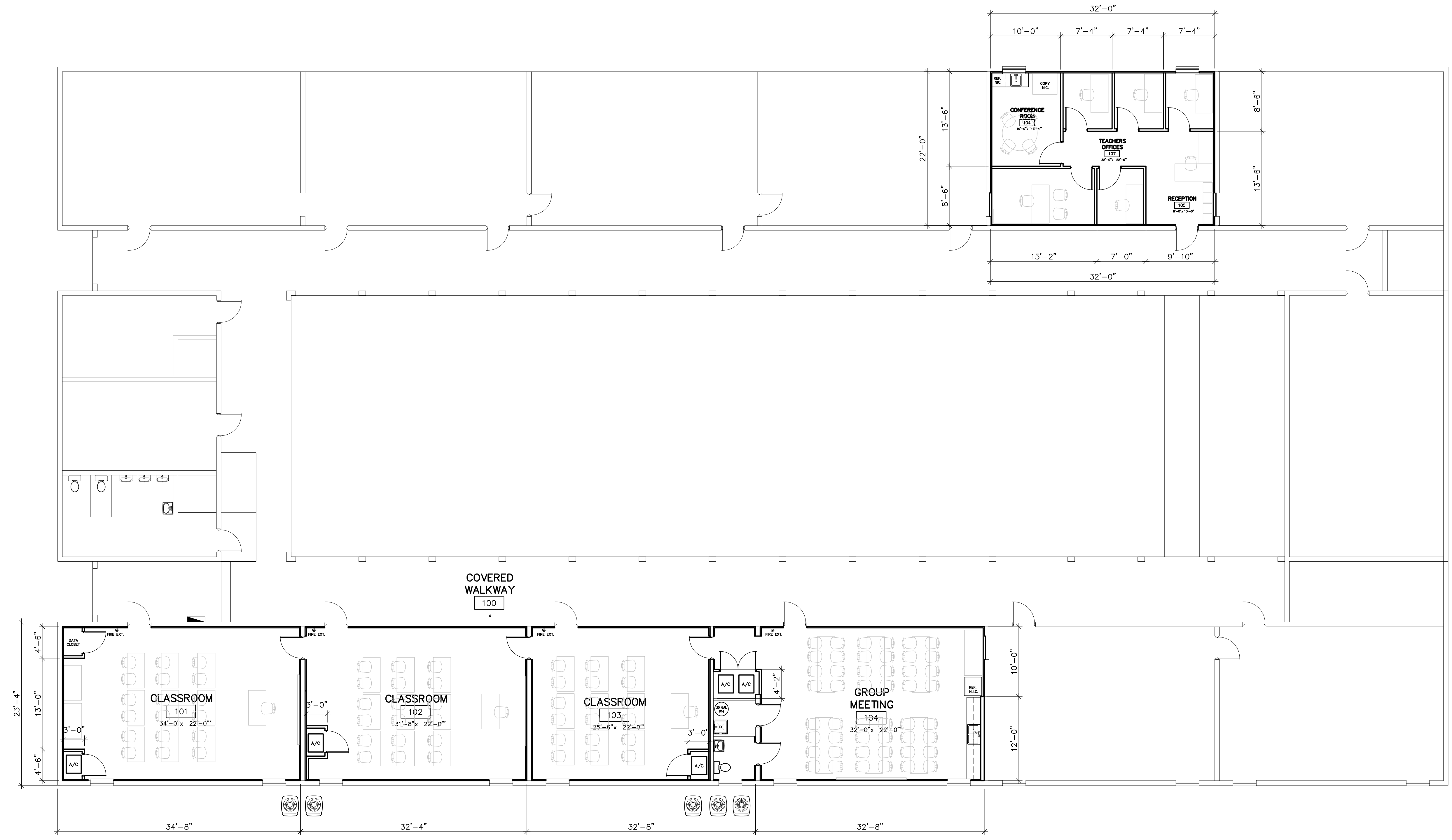
PROPOSED FLOOR PLAN 1/8" = 1'-0"
