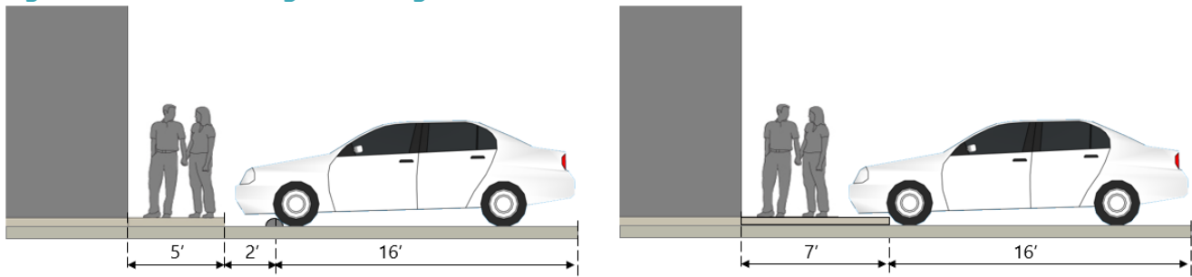
Figure VIII - 52. Parking Overhang
