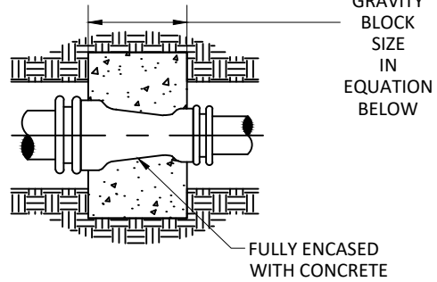
REDUCER
