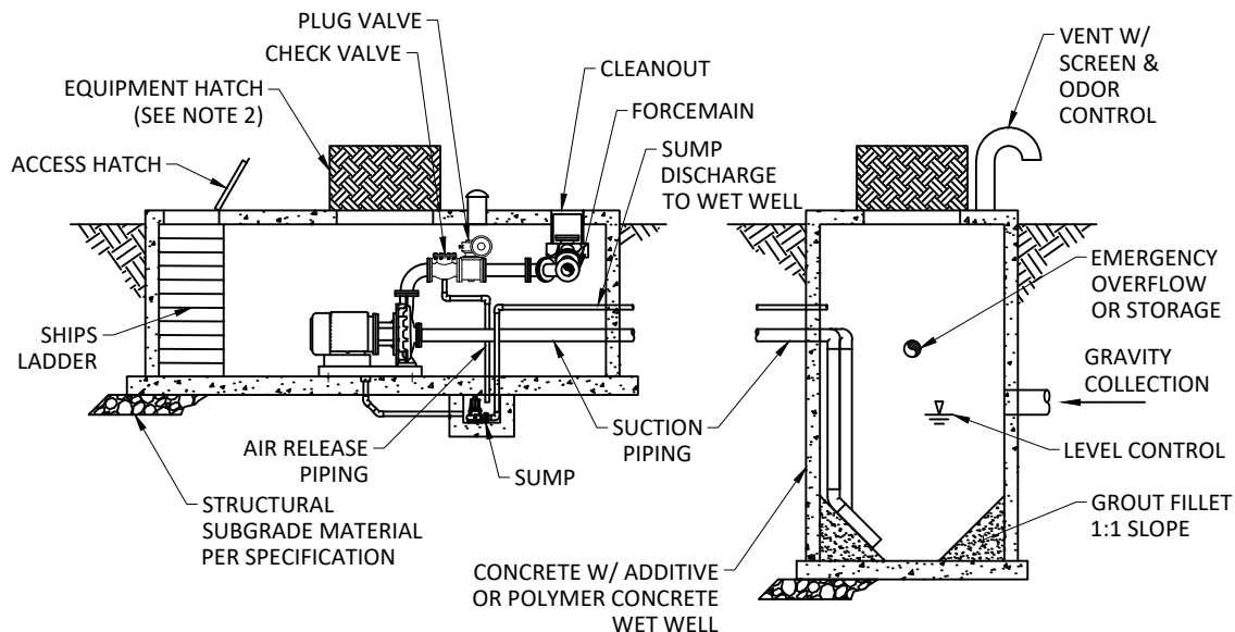
SECTION VIEW
