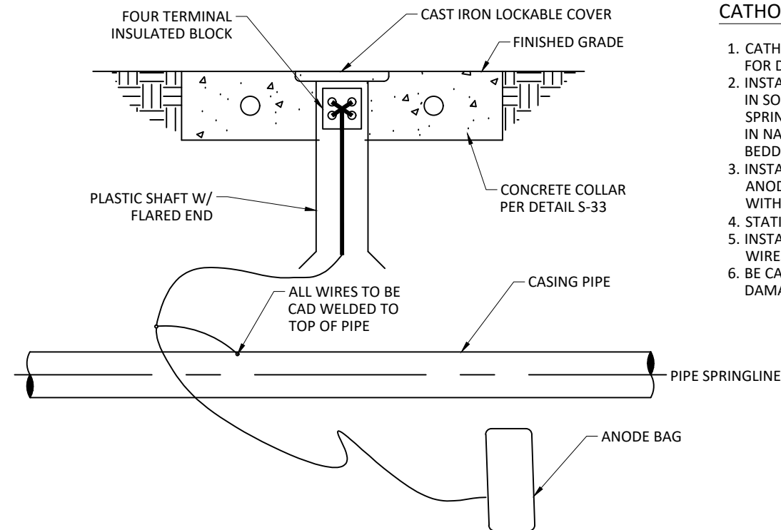
CATHODIC TEST STATION DETAIL
