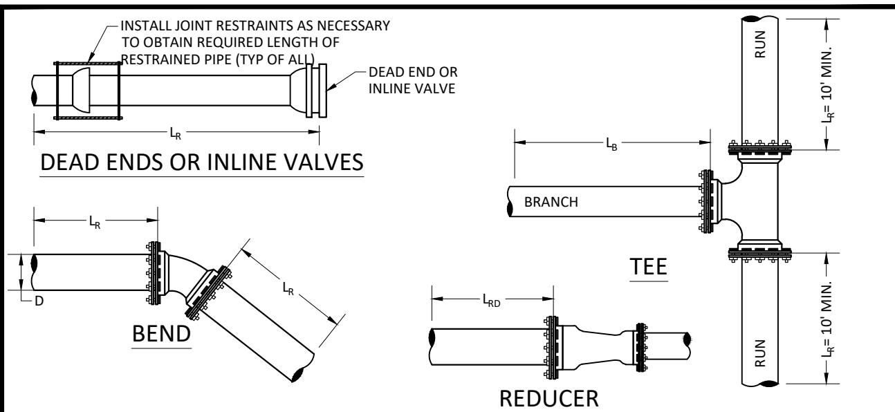
DI PIPE (POLYETHYLENE-ENCASED): MINIMUM LENGTHS OF RESTRAINED PIPE - IN FEET
