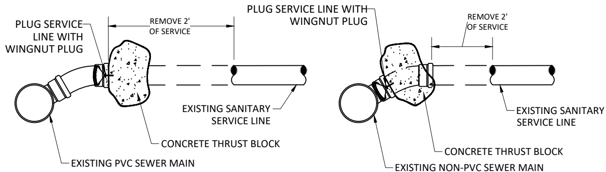
EXISTING SANITARY SEWER SERVICE ABANDONMENT DETAIL
