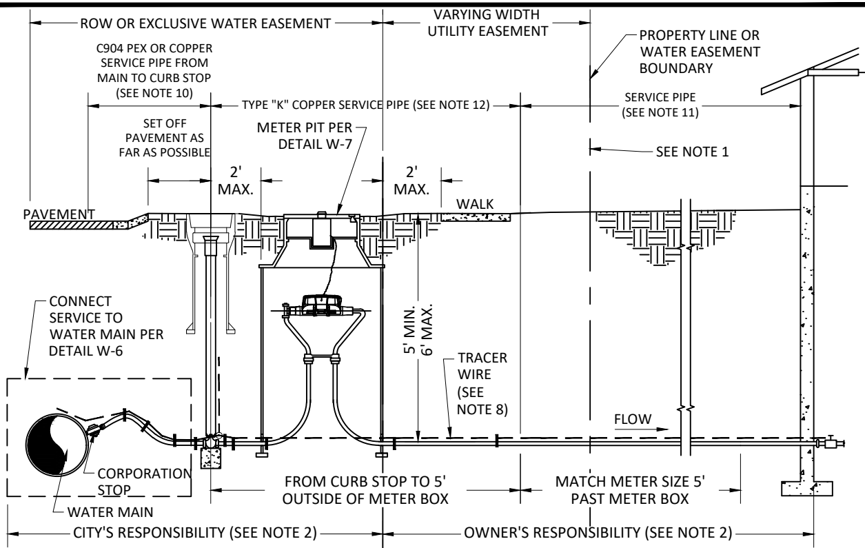
ELEVATION VIEW
