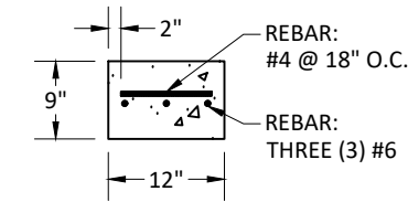
BASE BEAM DETAIL
