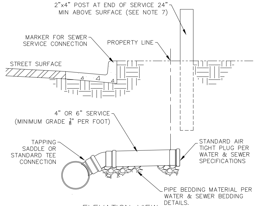
ELEVATION VIEW
