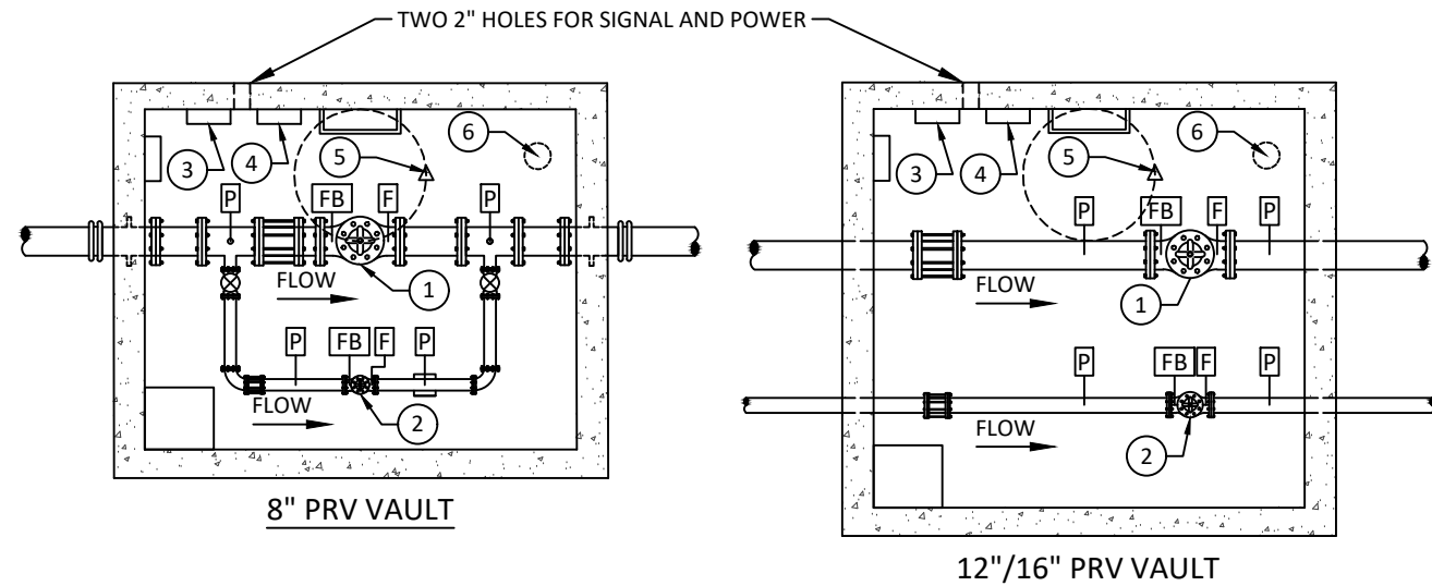
PLAN VIEWS
