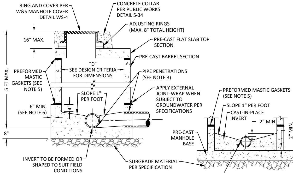
CAST-IN-PLACE BASE
