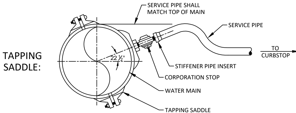
ELEVATION VIEW
