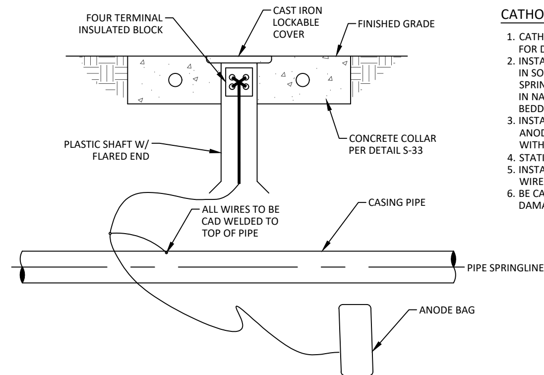
CATHODIC TEST STATION DETAIL
