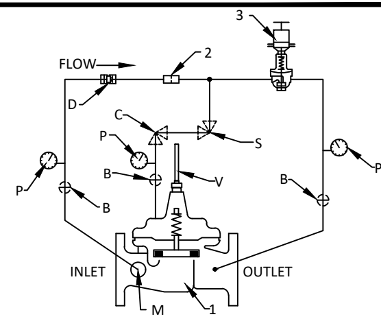
PRV COMPONENTS SCHEMATIC
