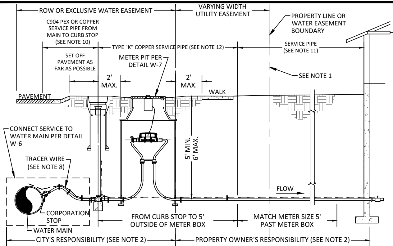
ELEVATION VIEW
