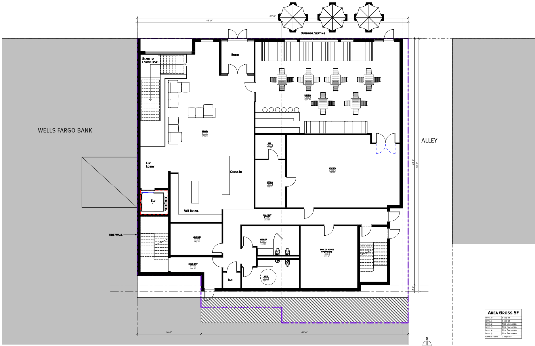
① LEVEL 1 FLOOR PLAN 3/16" = 1'-0"
