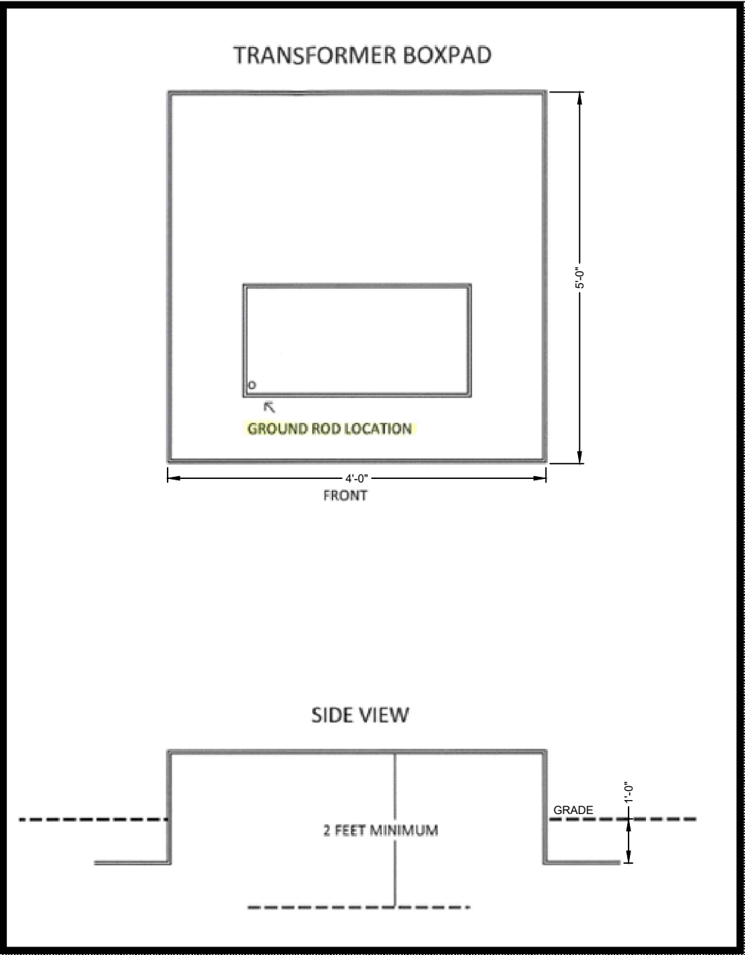
TRANSFORMER BOXPAD DETAIL
