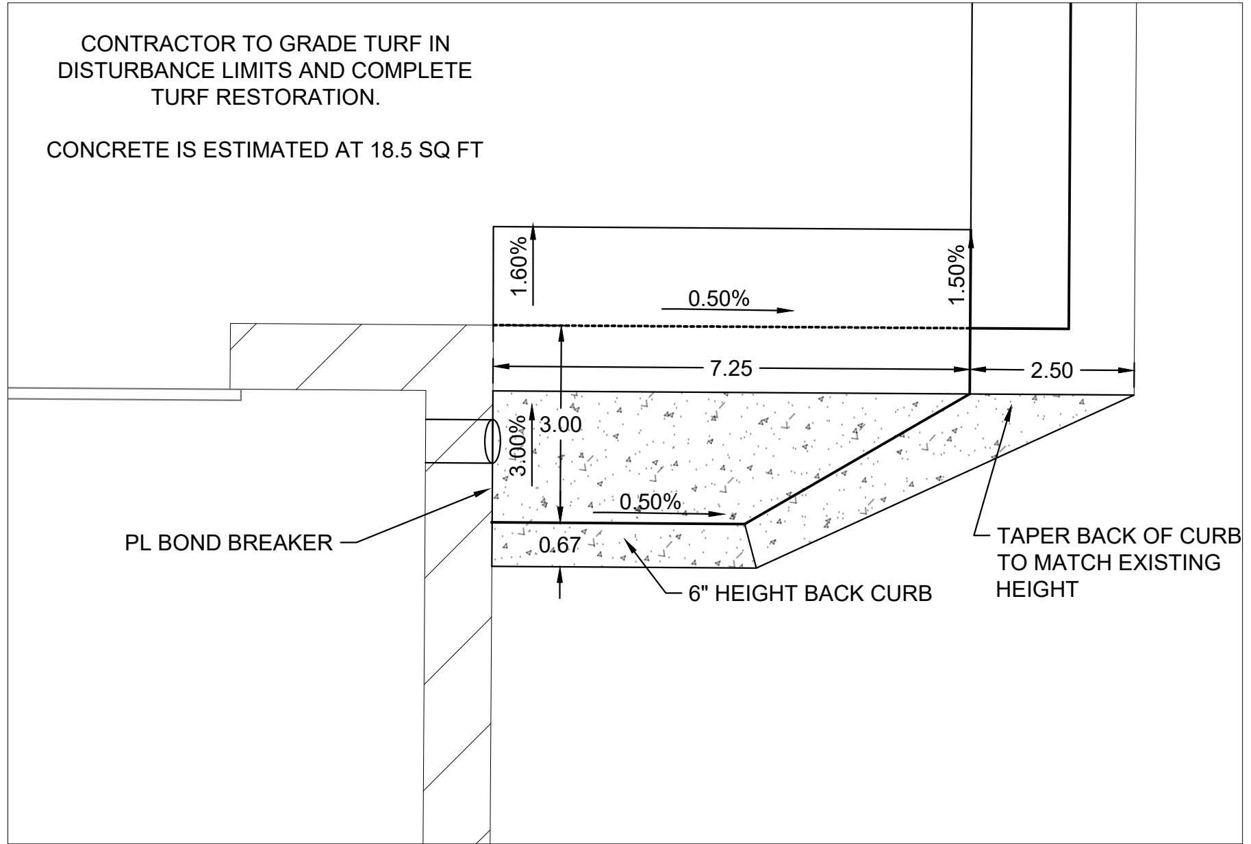
NORTHEAST OVERFLOW RAIN LEADER POURED IN PLACE SPLASH BLOCK
