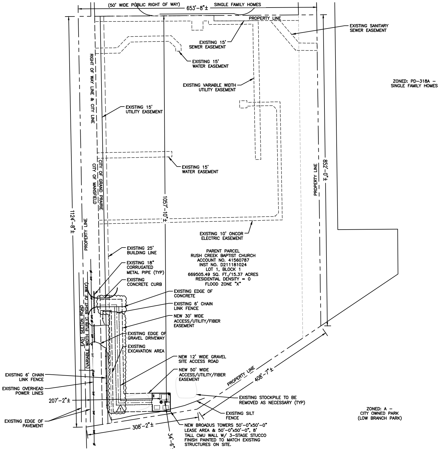
1 OVERALL SITE PLAN SCALE: 1" = 80'-0" (FULL SIZE) 1" = 160'-0" (11x17)
