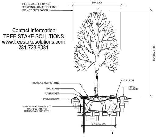
TREE PLANTING OVER 2" CALIPER SCALE: NOT TO SCALE
