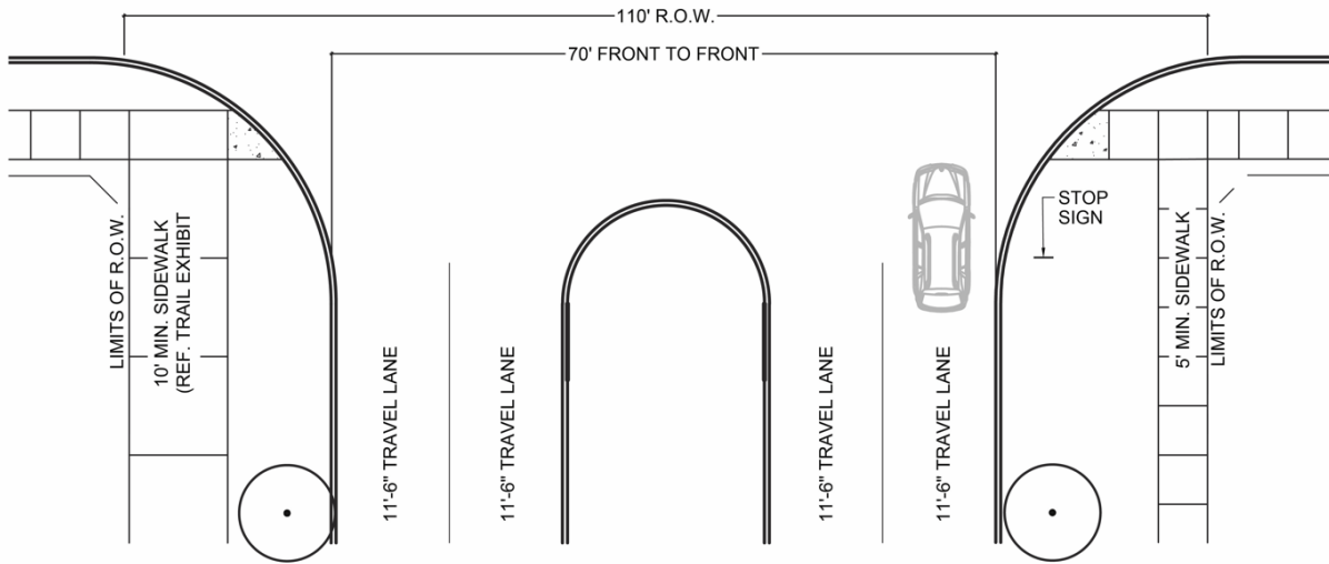
110' R.O.W. - 4 LANE DIVIDED MINOR ARTERIAL STREET INTERSECTION
