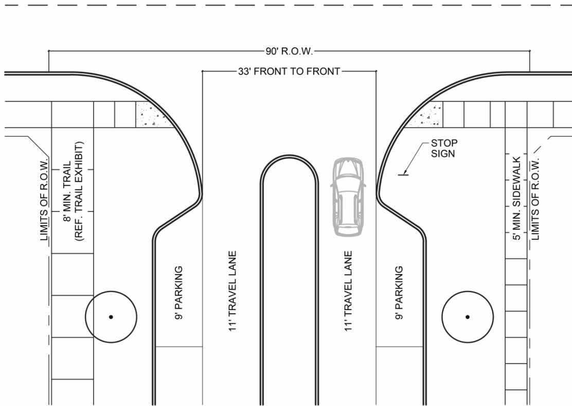
90' R.O.W. - RESIDENTIAL BOULEVARD STREET INTERSECTION
