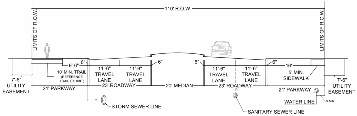
110' R.O.W. - 4 LANE DIVIDED MINOR ARTERIAL
