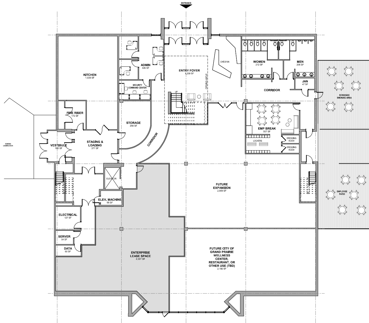
1 GROUND FLOOR PLAN CONCEPT **THIS DRAWING INDICATES THE CONCEPTUAL LAYOUT, FINAL DESIGN SUBJECT TO CHANGE 1/8" = 1'-0"
