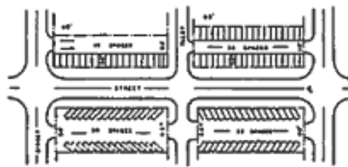
PARKING LAYOUT FOR 50' & 60' LOTS
