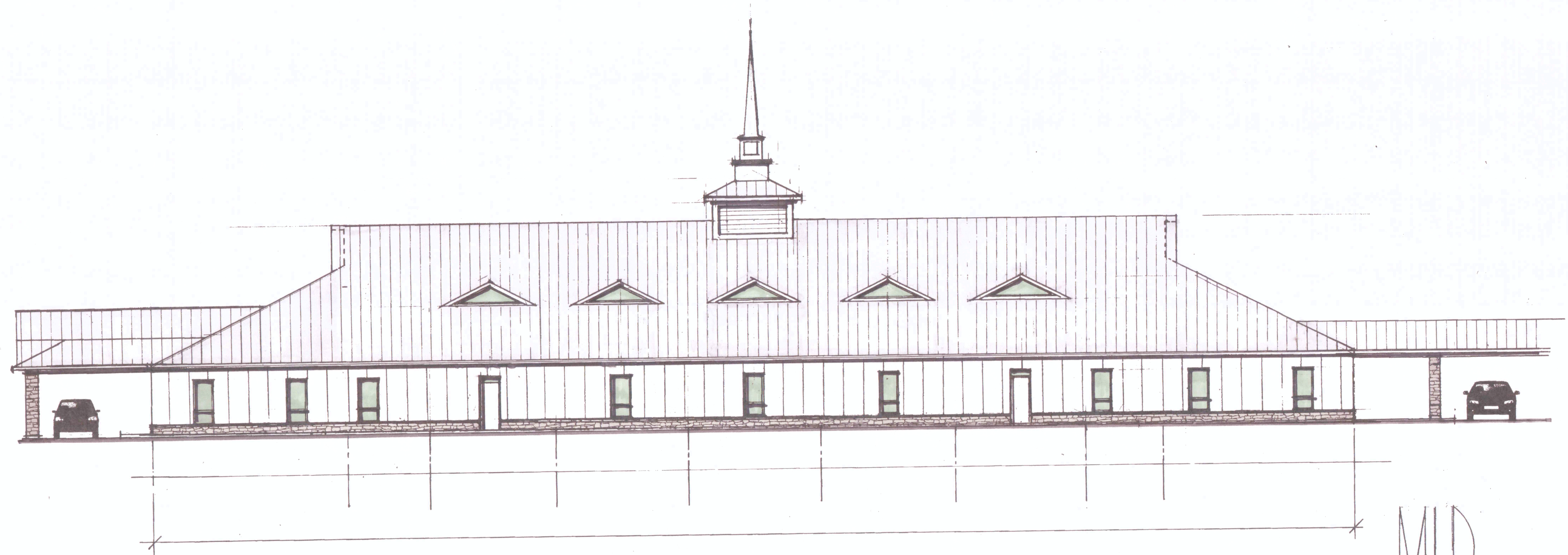
SOUTH ELEVATION 1/8" = 1'-0"
