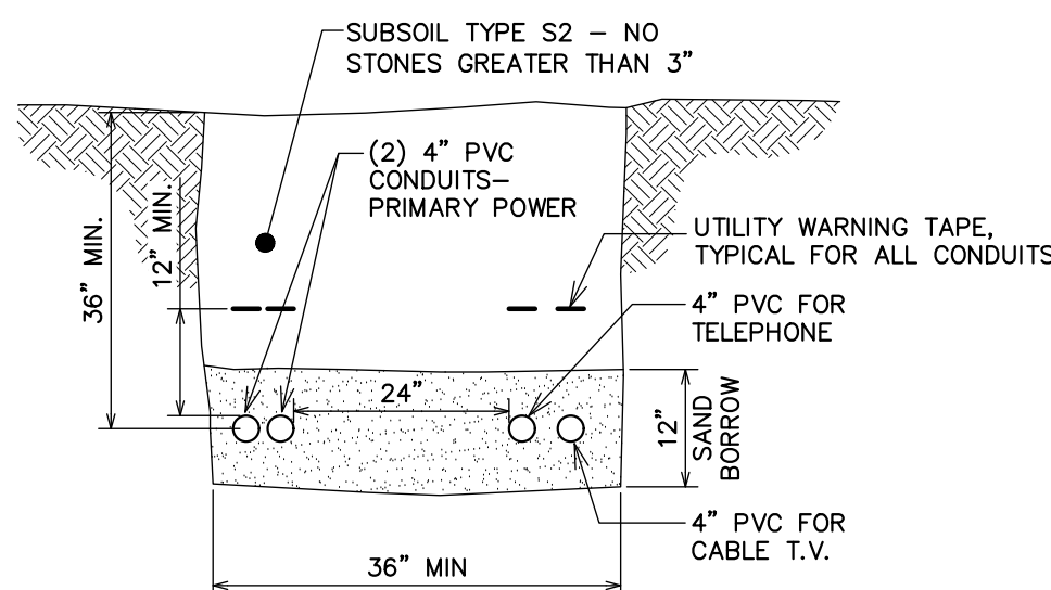
09 Utility Trench C-5 NOT TO SCALE
