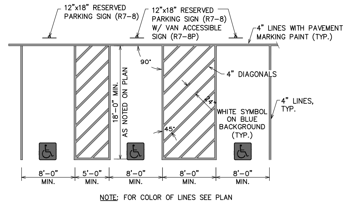
04 ADA Parking C-5 NOT TO SCALE
