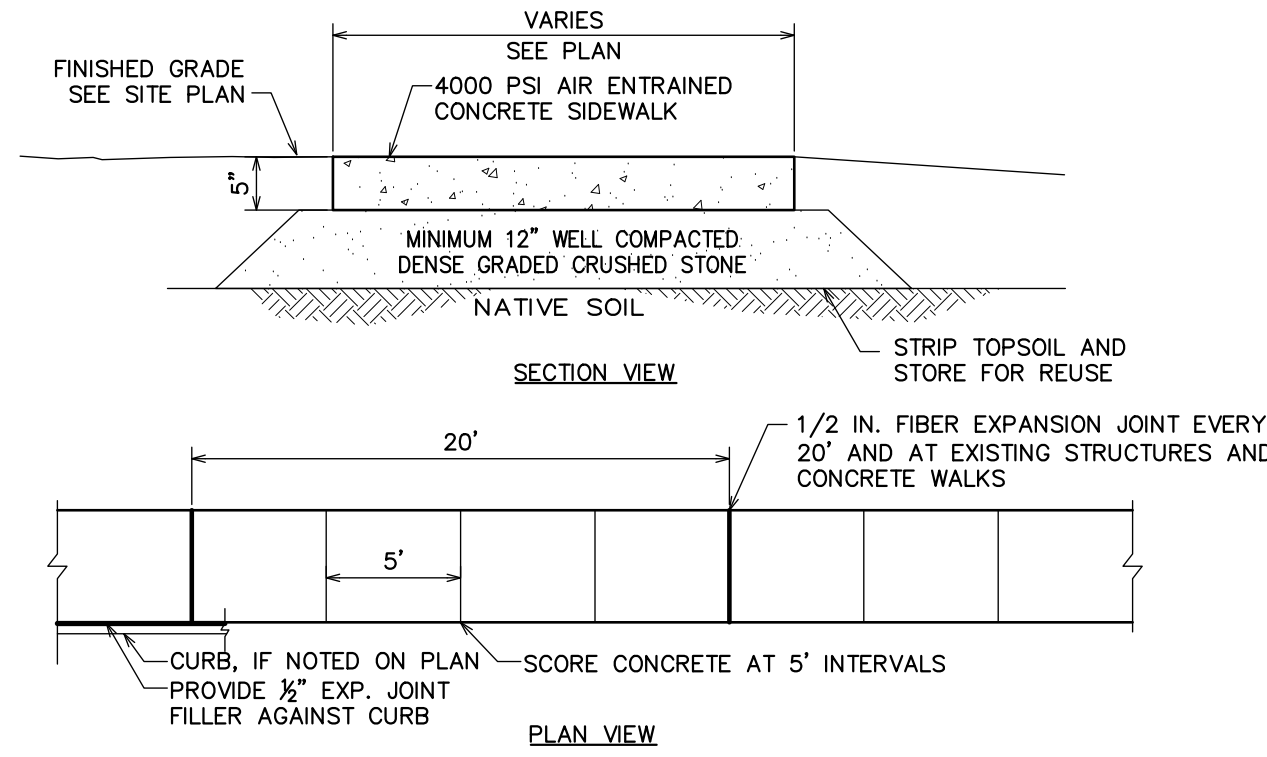
03 Concrete Sidewalk C-5 NOT TO SCALE
