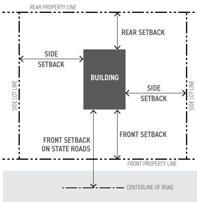
Figure 10.1 - Diagram of Lot Lines and Setbacks
