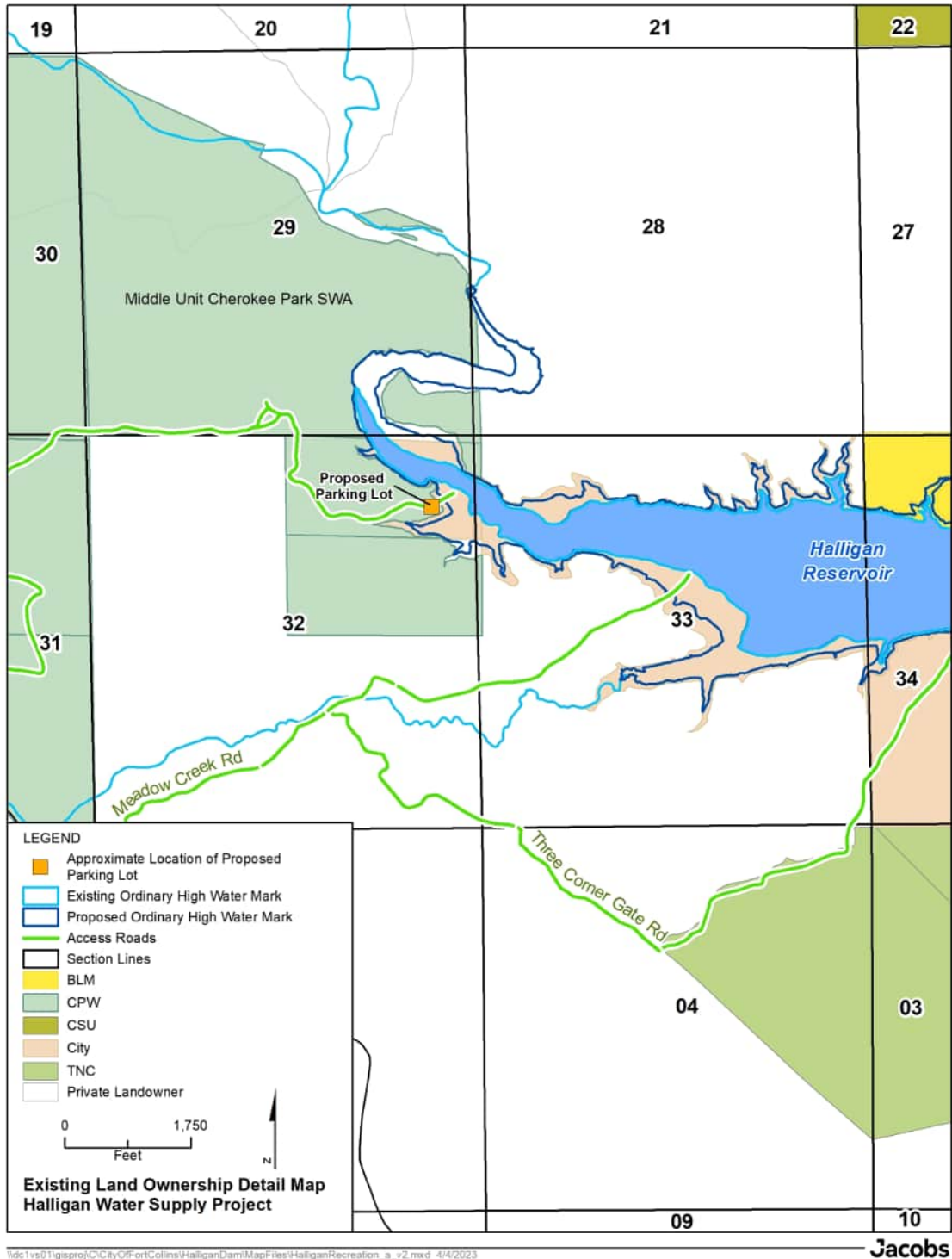
Figure 3-4. Sections 29 and 32 on the Western Edge of Halligan Reservoir
