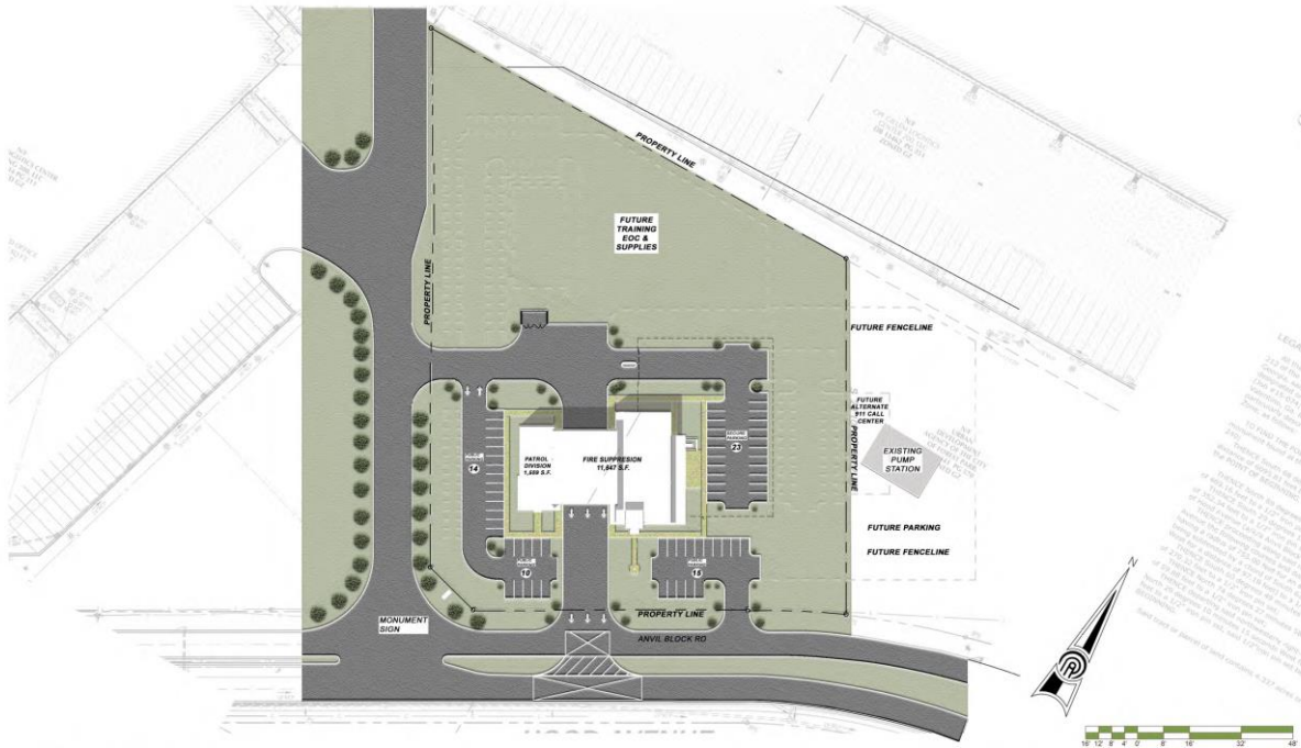
FOREST PARK GILLEM PUBLIC SAFETY FACILITY Design Development Site Plan SCALE: 1" = 80'-0" A21-006 05/13/2021
