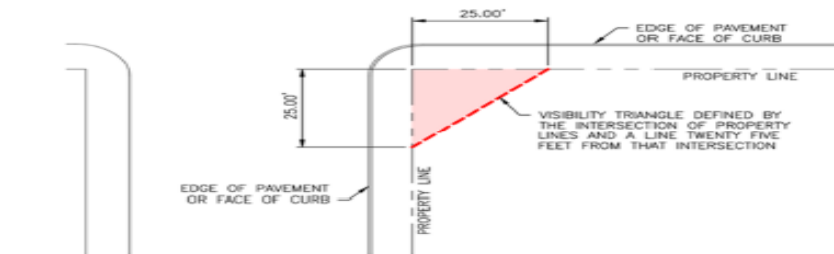
Figure. 6.1 Visibility Triangle
