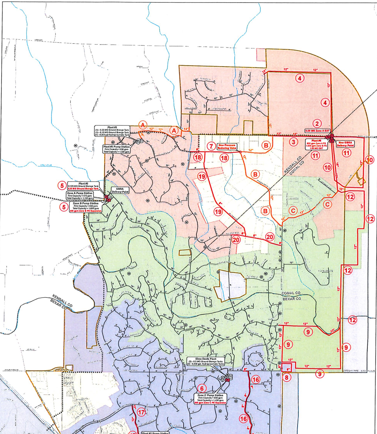
FIGURE 3-3 CITY OF FAIR OAKS RANCH WATER SYSTEM IMPACT FEE CAPITAL IMPROVEMENTS PLAN
