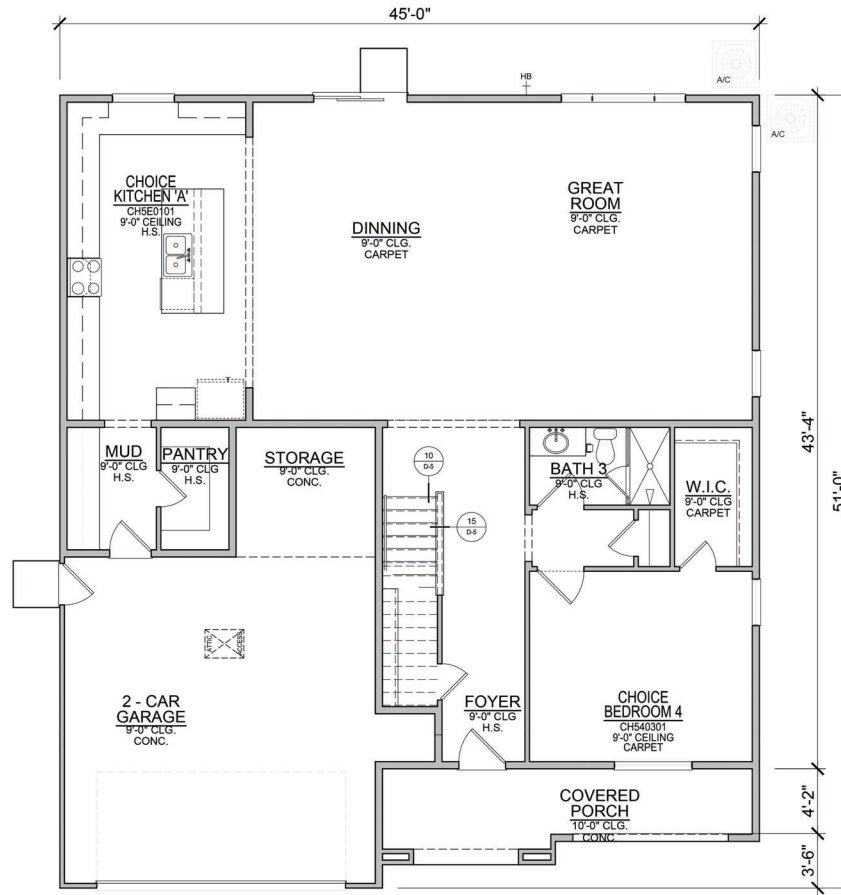
FIRST FLOOR PLAN - SCL - A SCALE: 1/8"=1'-0" (11"x17" SHEET SIZE) SCALE: 1/4"=1'-0" (22"x34" SHEET SIZE)
