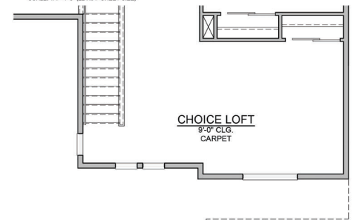
SECOND FLOOR PLAN - ACL - B SCALE: 1/8"=1'-0" (11x17" SHEET SIZE) SCALE: 1/4"=1'-0" (22x34" SHEET SIZE)
