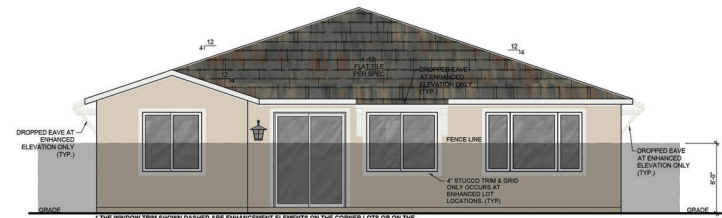
REAR ELEVATION - ACL - B SCALE: 1/8"=1'-0" (24"x36" SHEET SIZE)
