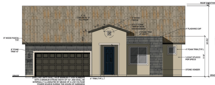
FRONT ELEVATION - ADL - C SCHEME 7 SCALE: 1/8"=1'-0" (11x17" SHEET SIZE) SCALE: 1/4"=1'-0" (24x36" SHEET SIZE)
