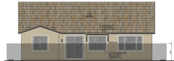
REAR ELEVATION - ADL - C SCALE: 1/4"=1'-0" (24"X36" SHEET SIZE)
