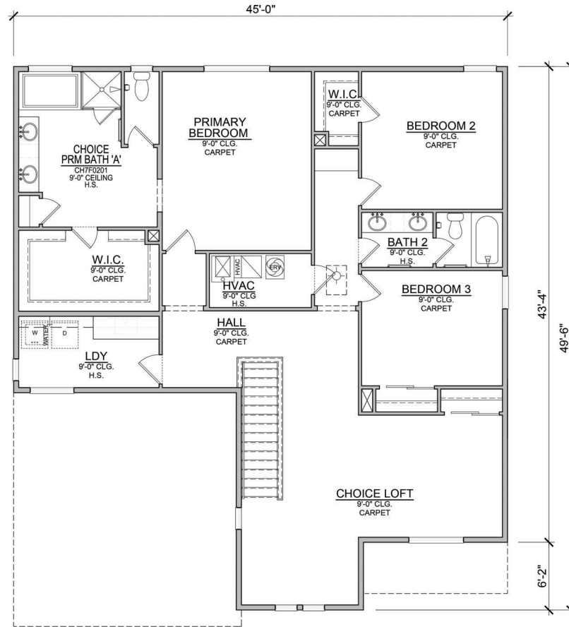
SECOND FLOOR PLAN - SCL - A SCALE: 1/8"=1'-0" (11x17" SHEET SIZE) SCALE: 1/4"=1'-0" (22x34" SHEET SIZE)
