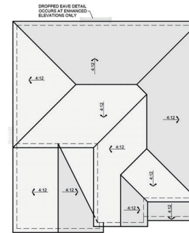
ROOF PLAN - SCL - A SCALE: 1/8"=1'-0" (11 1/16" SHEET SIZE) SCALE: 1/4"=1'-0" (24"x36" SHEET SIZE)
