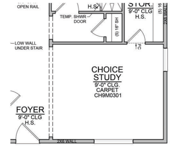
CHOICE STUDY SCALE: 1/8"=1'-0" (11"x17" SHEET SIZE) SCALE: 1/4"=1'-0" (22"x34" SHEET SIZE)
