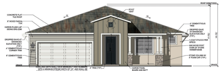
FRONT ELEVATION - ACL - B SCHEME 4 SCALE: 1/8"=1'-0" (11x17" SHEET SIZE) SCALE: 1/4"=1'-0" (24x36" SHEET SIZE)
