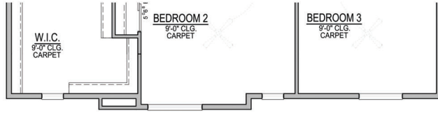
SECOND FLOOR PLAN - ACL - B
