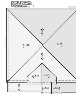
ROOF PLAN - SCL - A SCALE: 1/8\"/>
