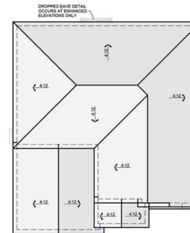
ROOF PLAN - ADL - C SCALE: 1/8"=1'-0" (24"X36" SHEET SIZE)
