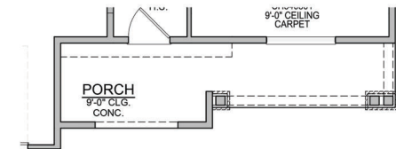
FIRST FLOOR PLAN - ACL - B SCALE: 1/8"=1'-0" (11"x17" SHEET SIZE) SCALE: 1/4"=1'-0" (22"x34" SHEET SIZE)
