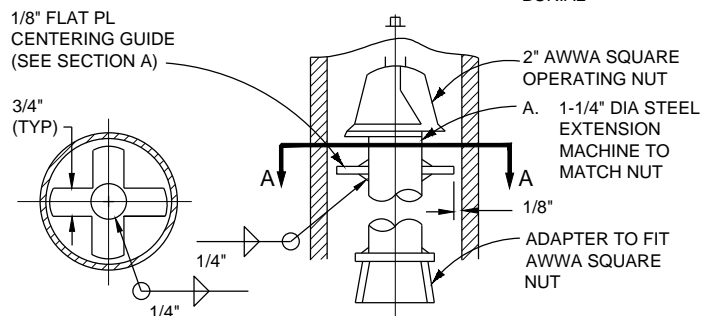
SECTION A
