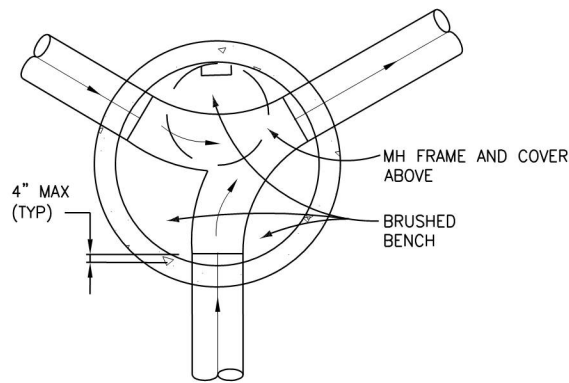
TYPICAL PLAN
