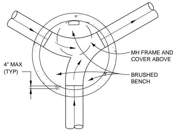
TYPICAL PLAN
