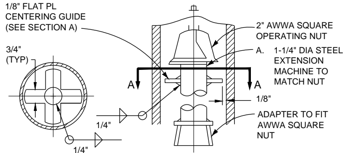
SECTION A
