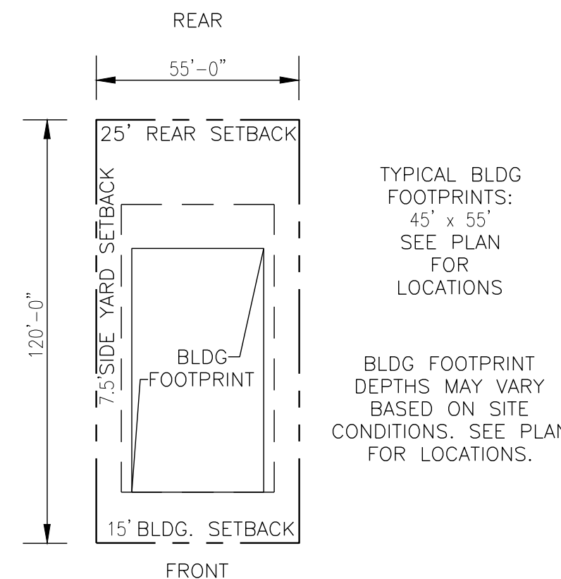
TYPICAL LOT LAYOUT SINGLE FAMILY NOT TO SCALE
