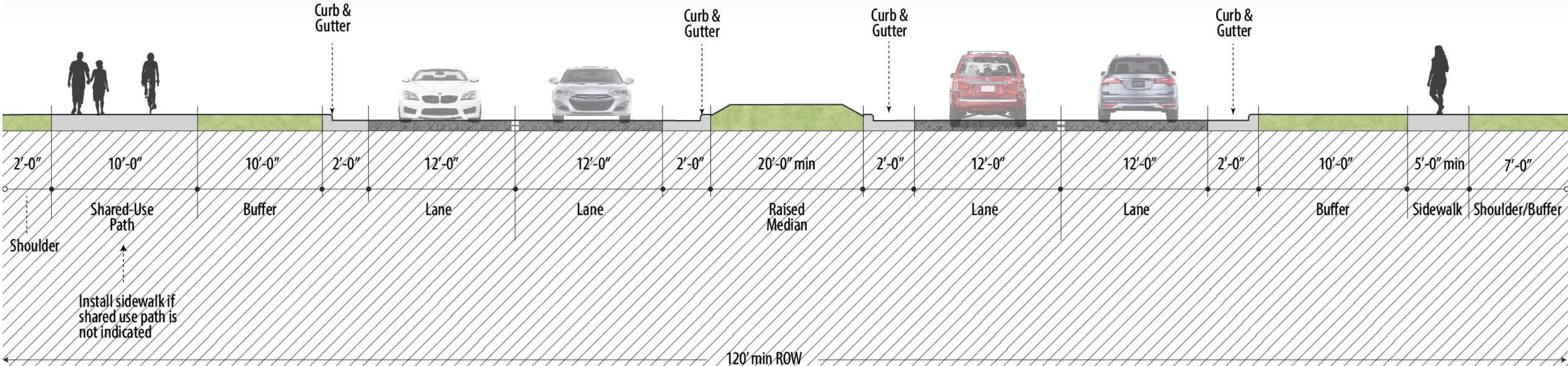
Arterial - Urban Road Cross Section (45 MPH TYP.)
