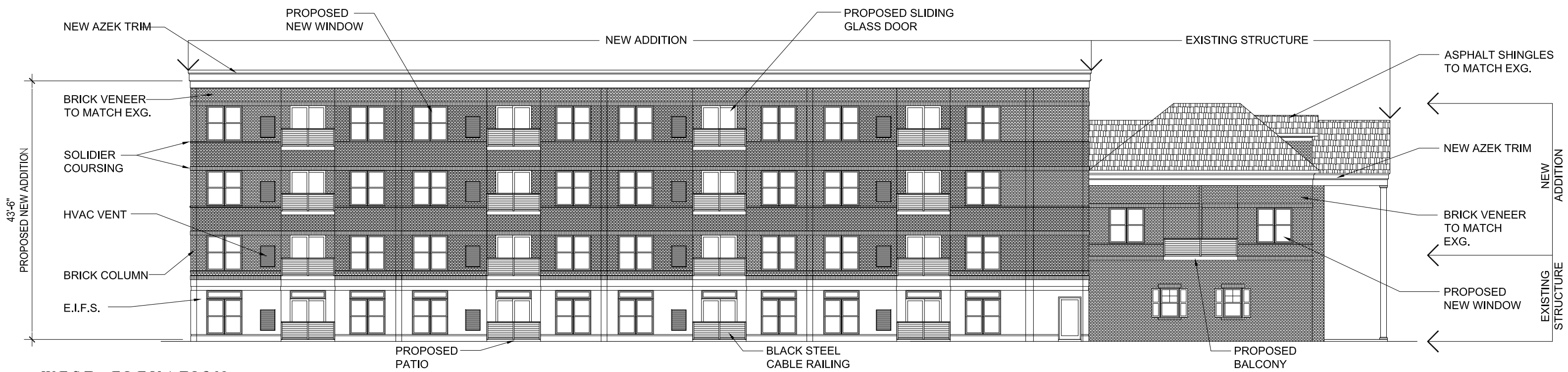
WEST ELEVATION
