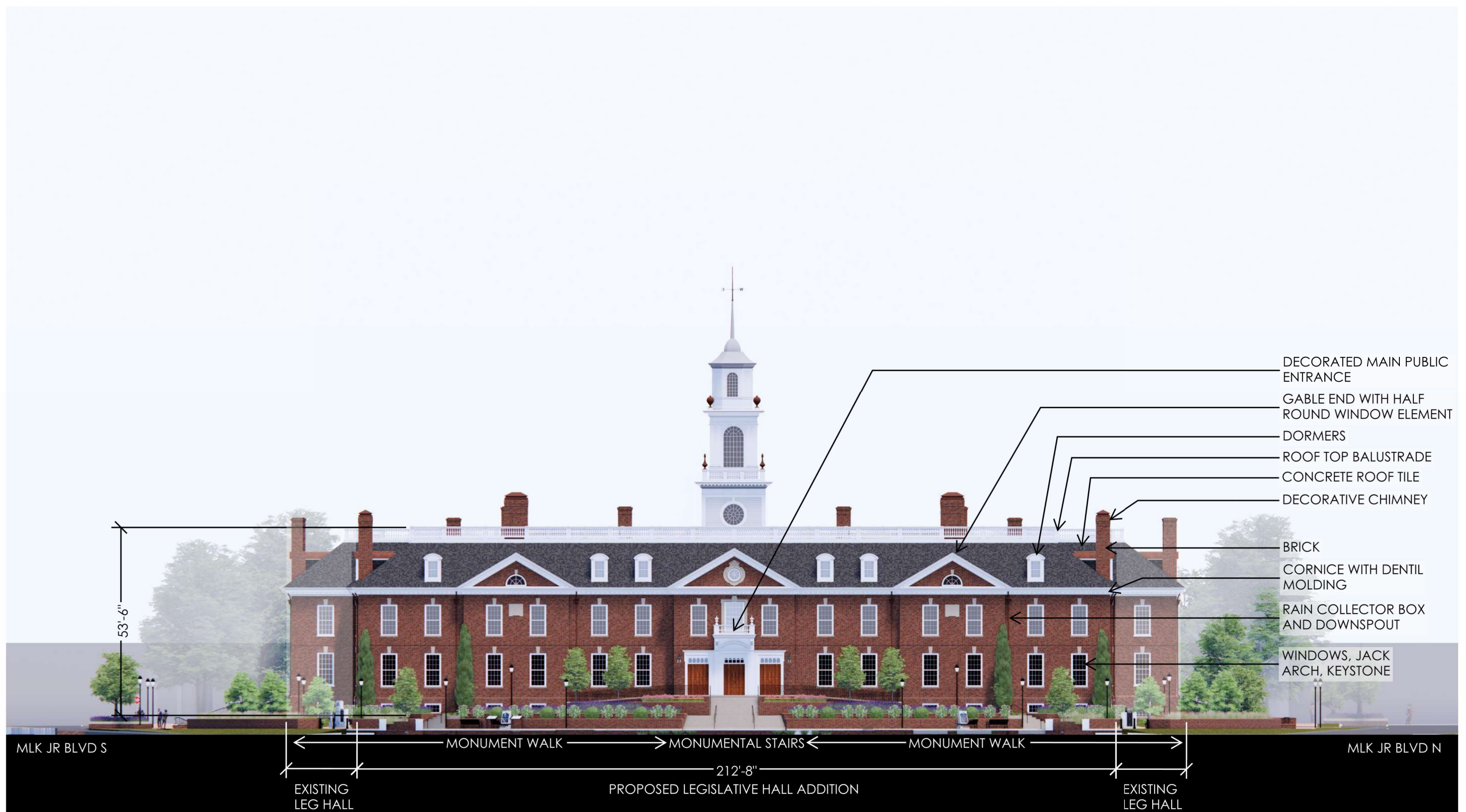
B-B - ELEVATION WESTBOUND FROM US-13 ON MLK JR BLVD
