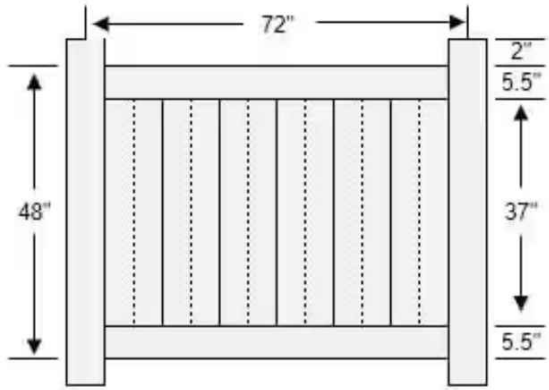
DETAIL: 4' HIGH VINYL TRASH ENCLOSURE SCALE: NONE
