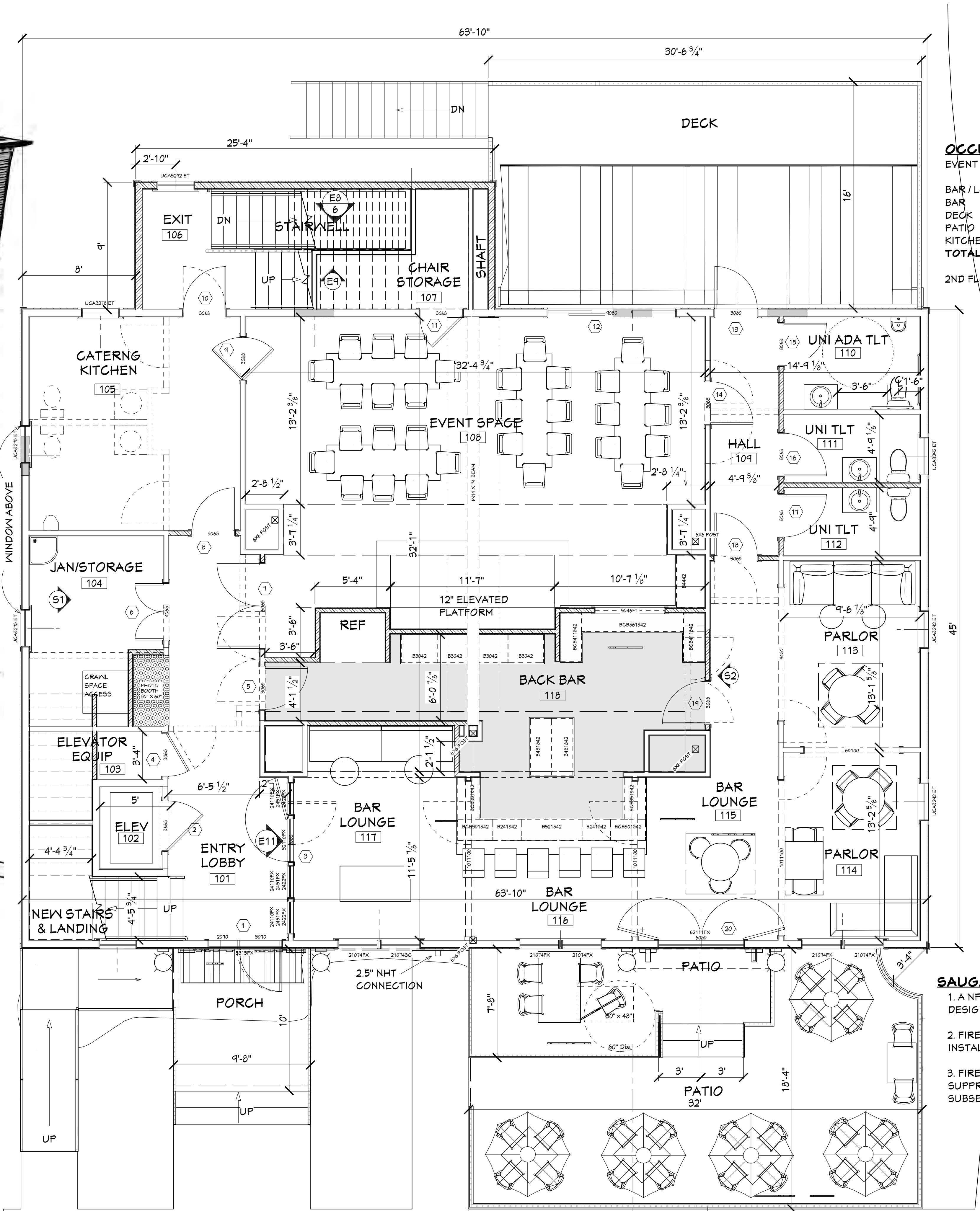
FIRST FLOOR PLAN SCALE: 1/4" = 1'-0" NEW TOTAL FLOOR AREA 3,101 S.F. 2,873 SQ. FT. ORIGINAL BUILDING
