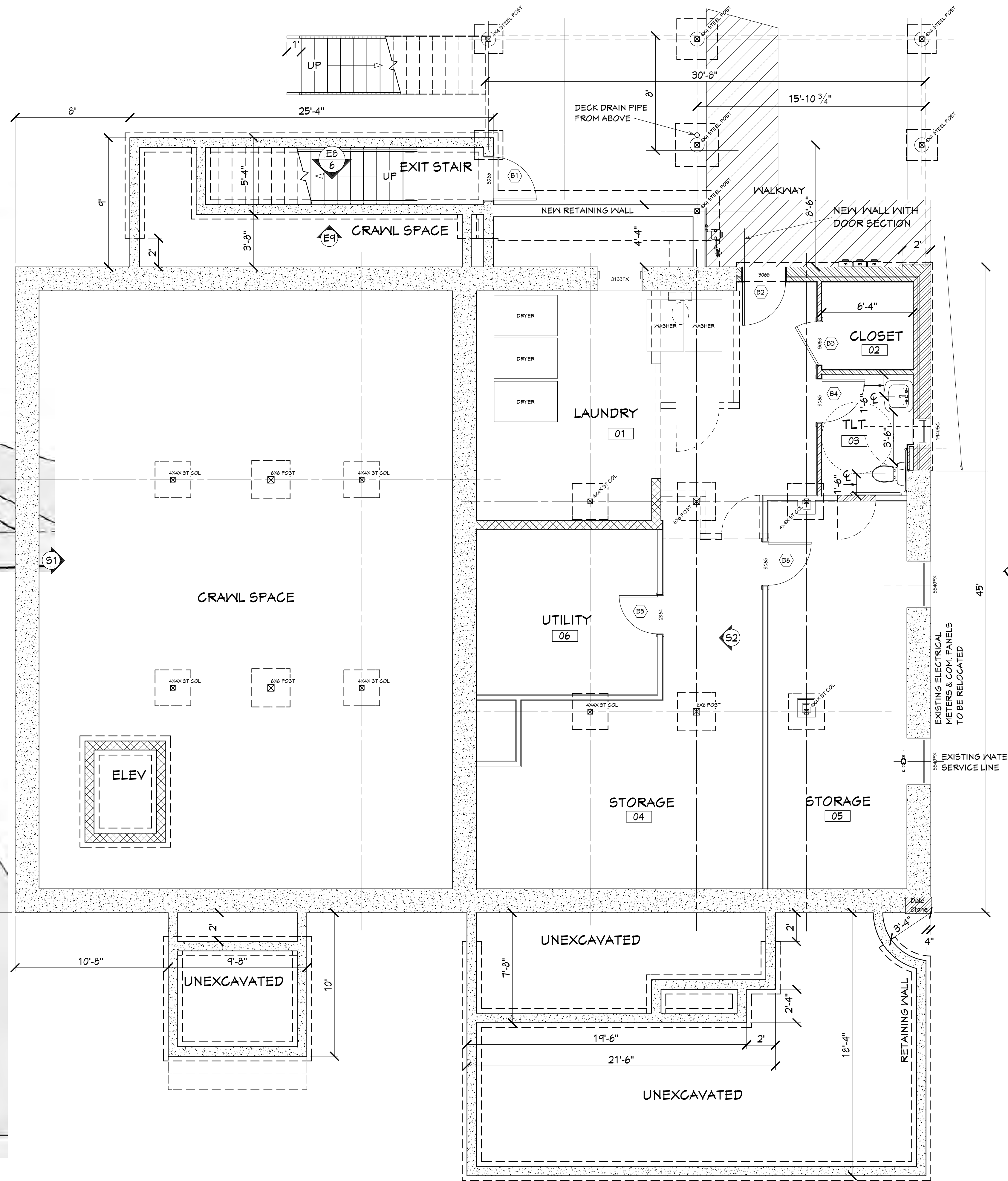
BASEMENT PLAN FLOOR AREA 1,463 S.F. SCALE: 1/4" = 1'-0"
