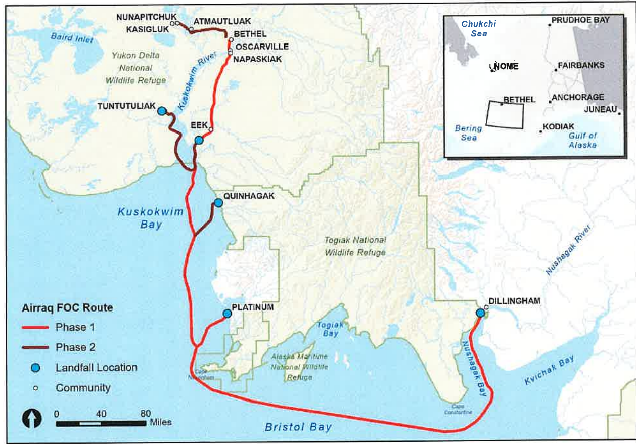
Airraq Network Overview Map
