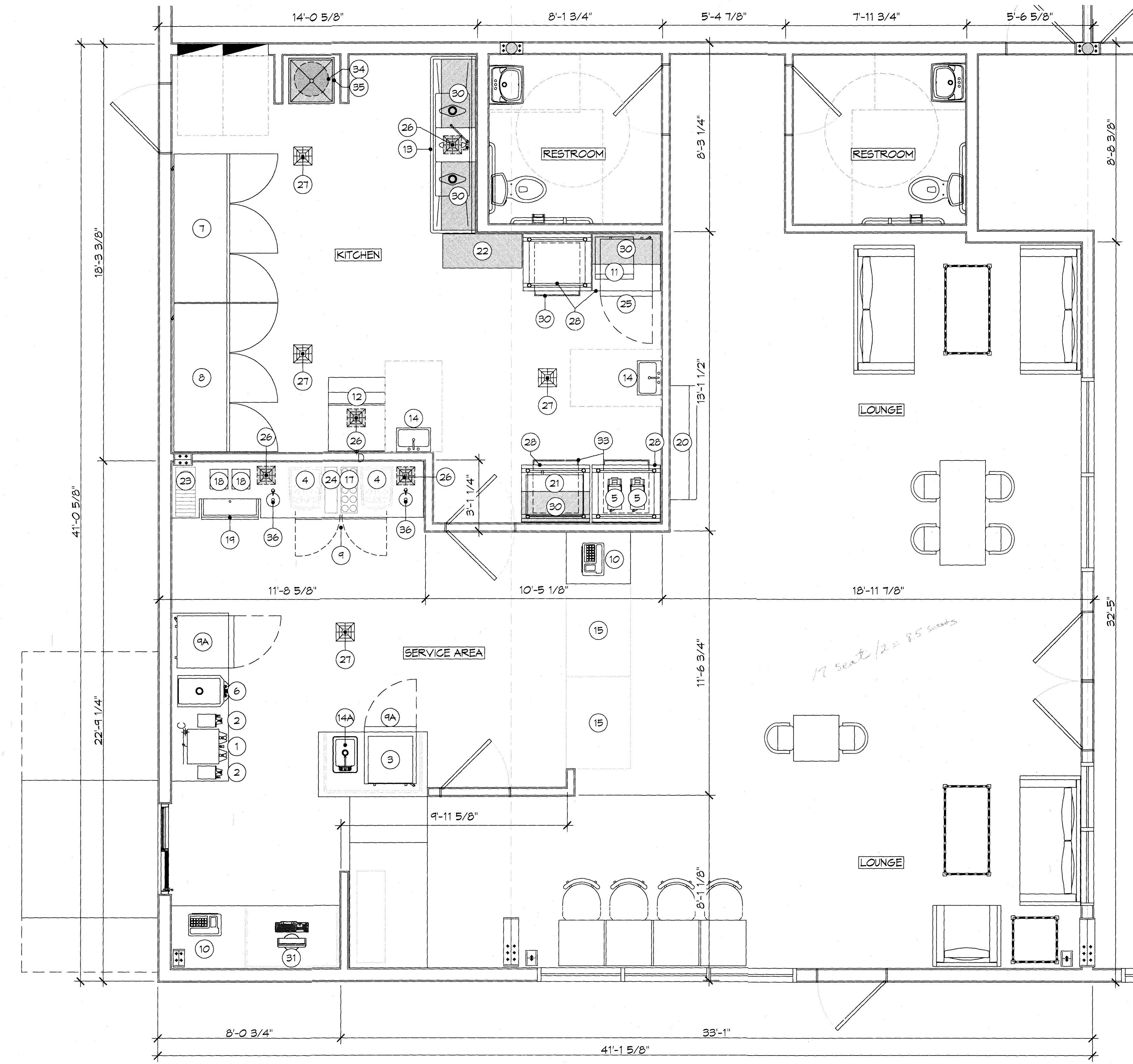
PJ'S FLOOR PLAN SCALE: 3/8" = 1'-0"
