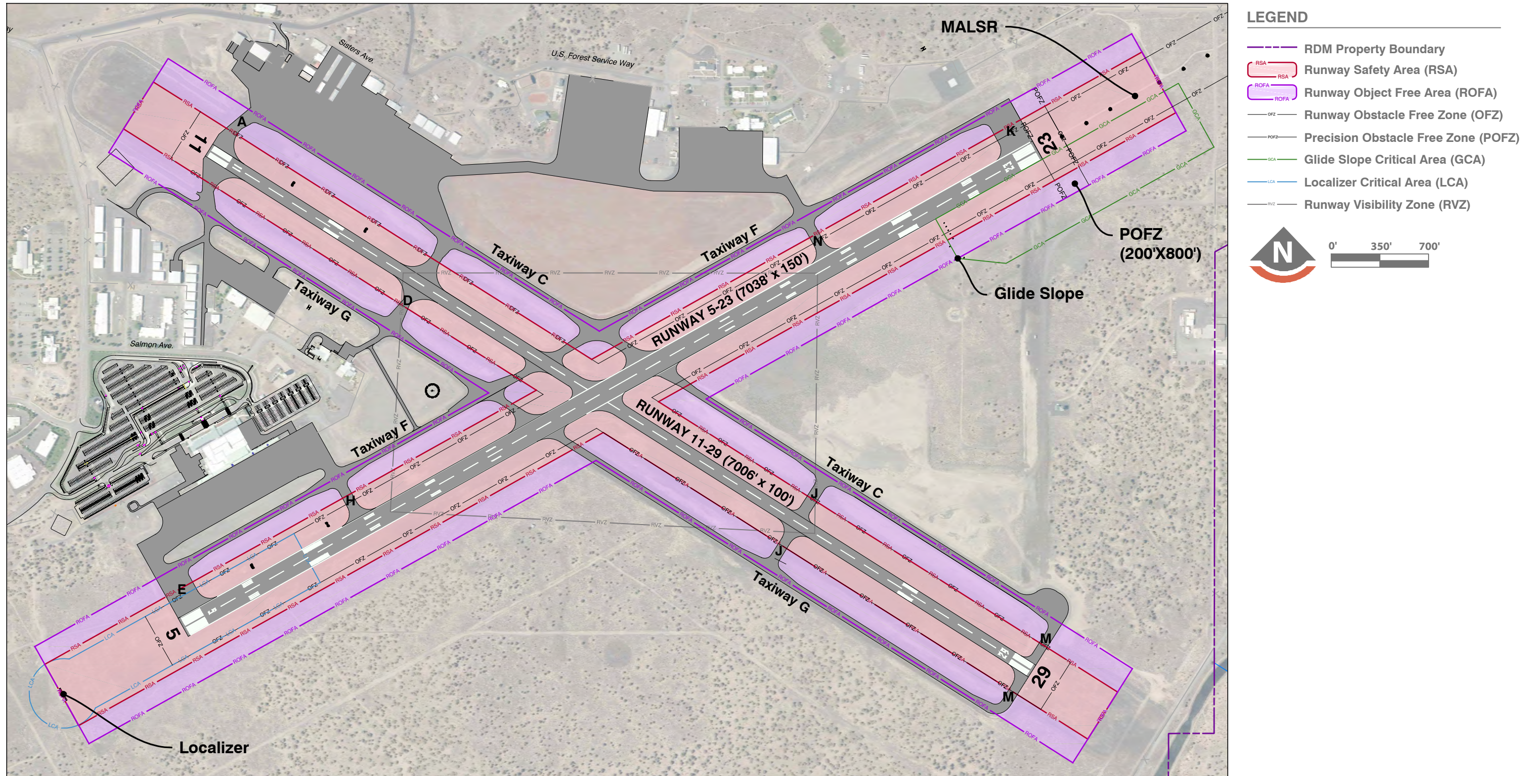
Figure 3-3 RUNWAY DESIGN SURFACES
