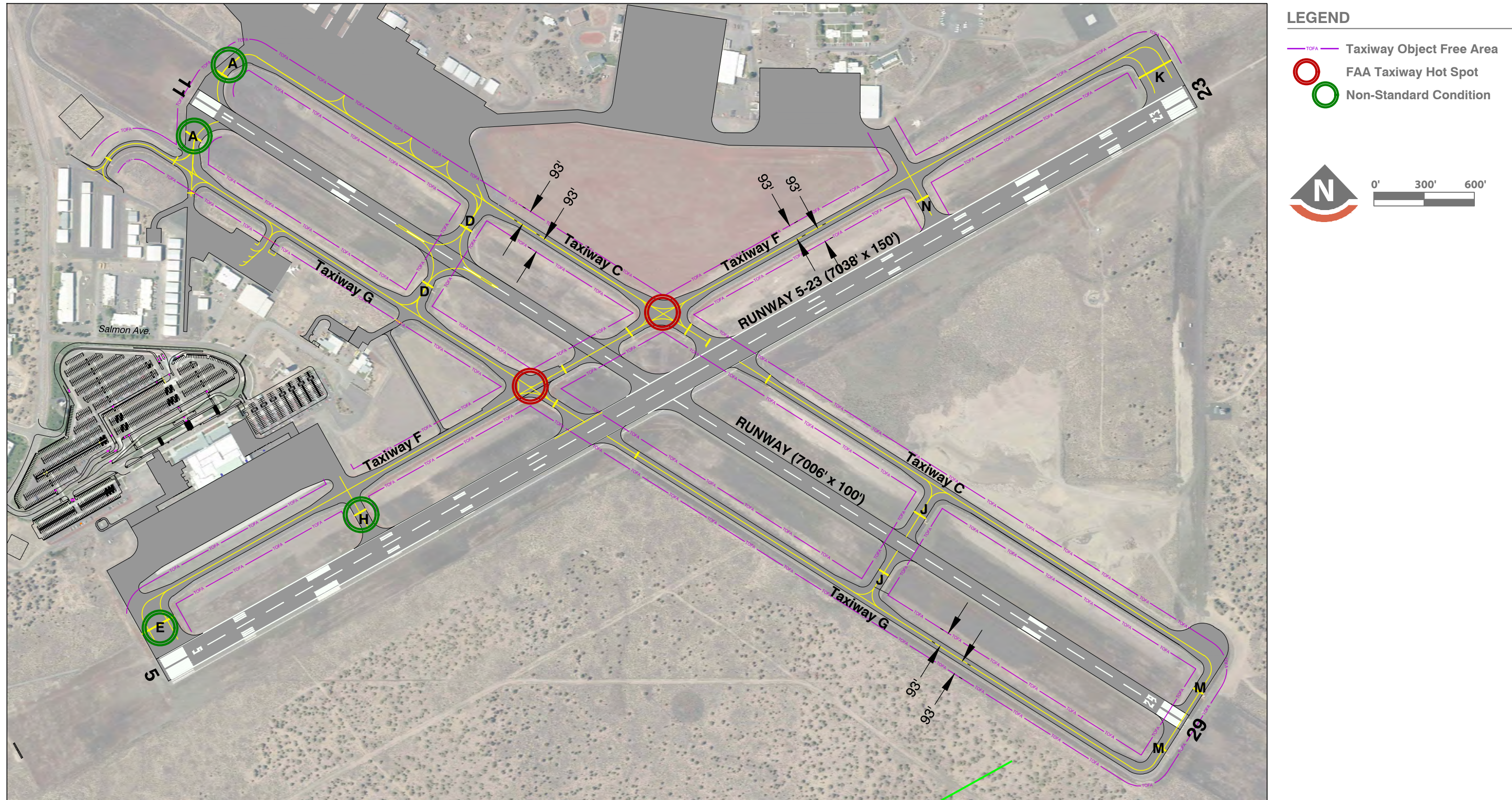
Figure 3-13 TAXIWAY DESIGN
